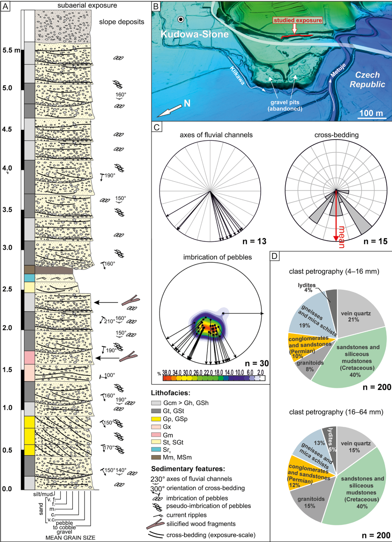
Fig. 3. Lithofacies succession, location, palaeoflow indicators and clast composition of the Kudowa-Stone deposits. A. Sedimentological log from the Kudowa-Stone exposure, with lithofacies and other sedimentary features indicated. B. Detailed location of the study site, shown on a 3D block diagram, generated from LiDAR data, viewed toward the ESE. C. Rose diagrams illustrating the measured
