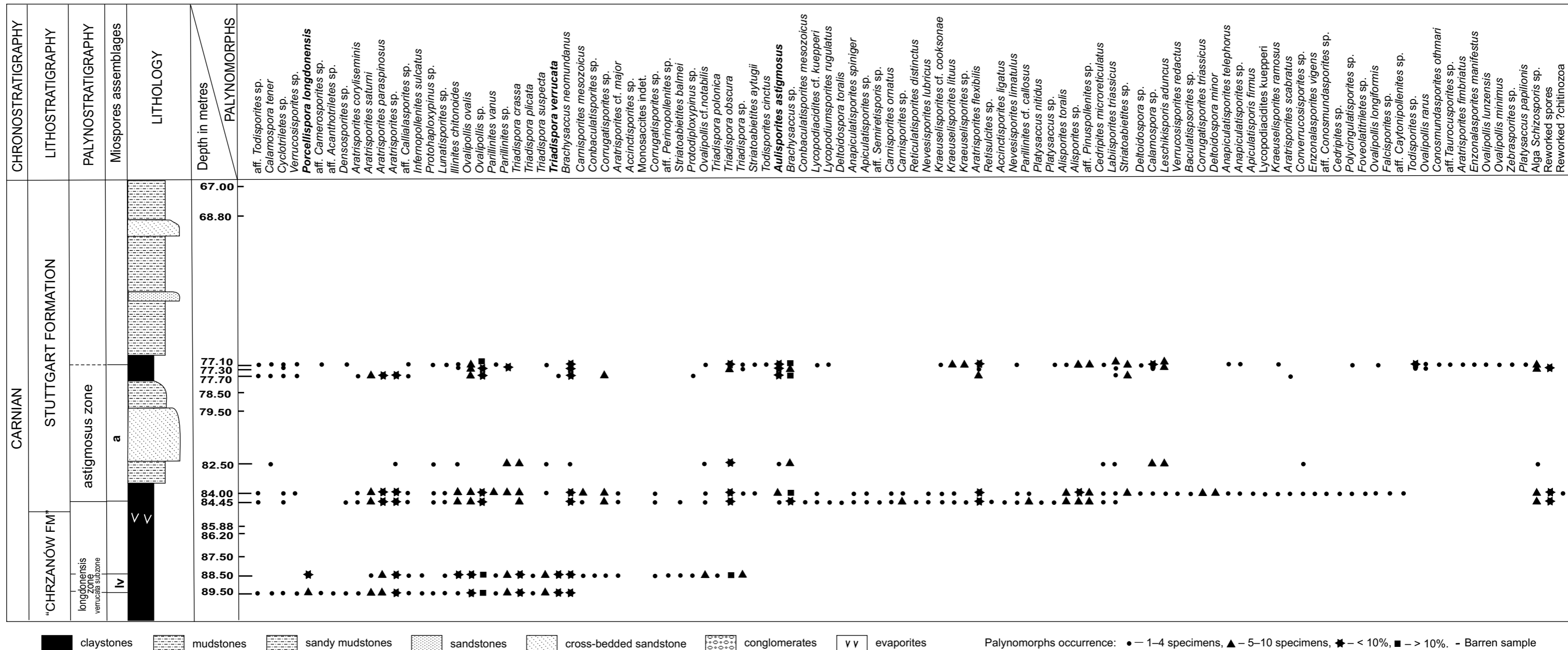
Fig. 3. Miospore occurrence in the Woźniki K1 borehole (names of index species are in bold print).
