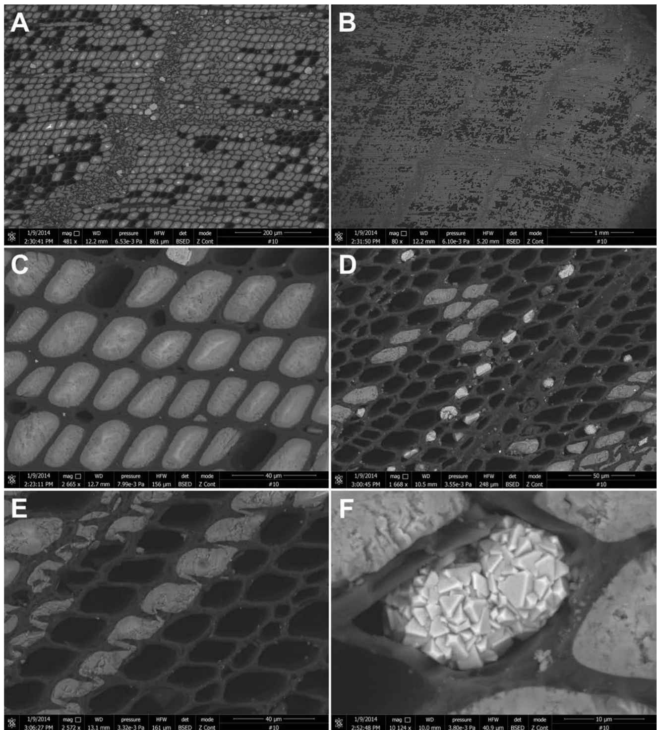
Fig. 3. Cut and polished charcoal (PORHA) from the Pořeba site under SEM. A. Wood filled with calcite, exhibiting a tangentially oriented zones of compressed cells. B. Wood filled with calcite, exhibiting tangentially oriented zones of compressed cells. C. Tracheids filled with calcite in close up. D. Mixture of empty tracheids and tracheids filled with calcite and pyrite. E. Zipper-like structure, cell lumina filled with calcite. F. Close up of tracheid cell filled with recrystallized pyrite framboid.
