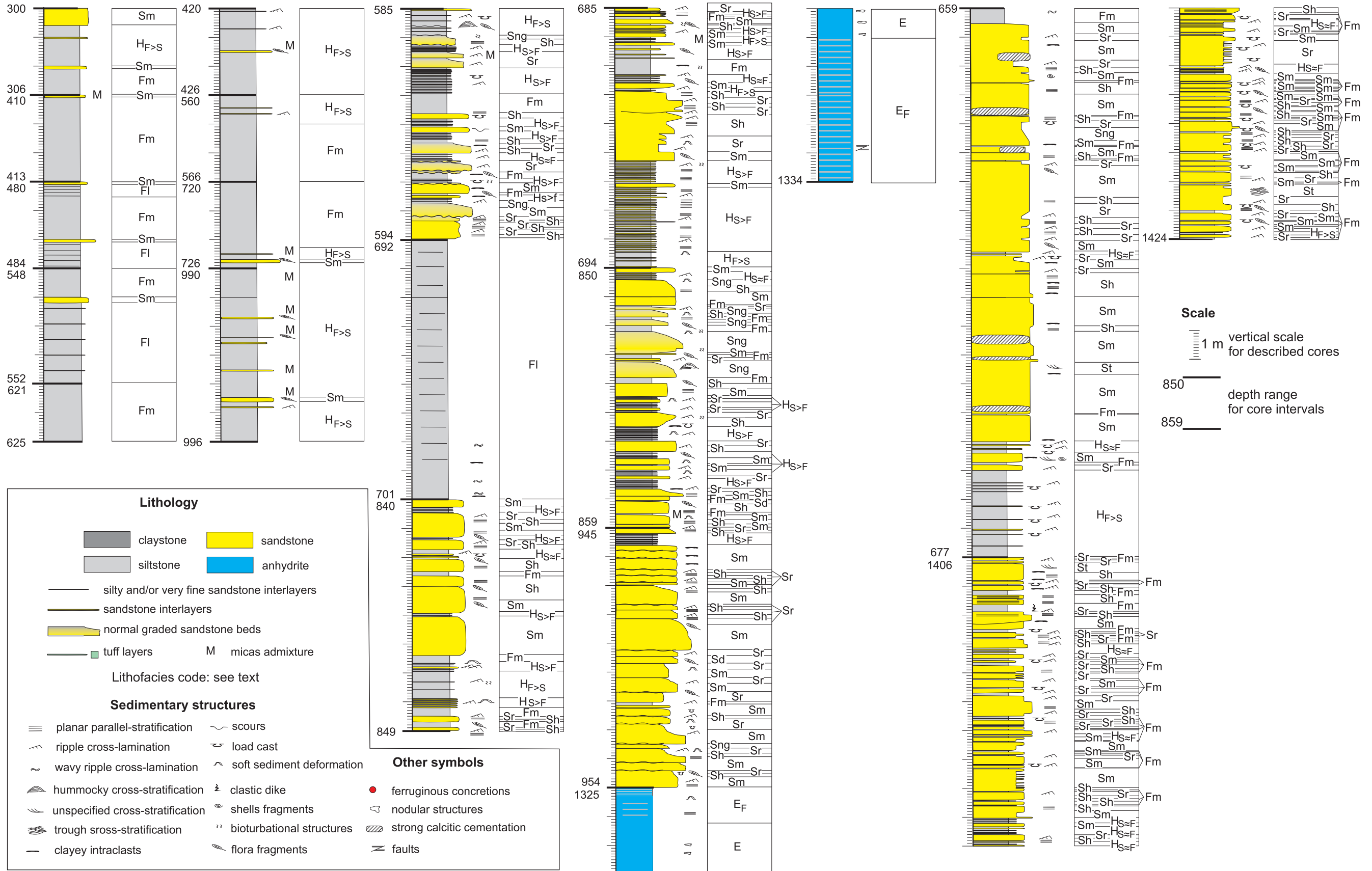
Fig. 6. Facies well logs of mid-Miocene, sedimentary succession in Polish part of Carpathian Foredeep (for well locations, see Fig. 1)
