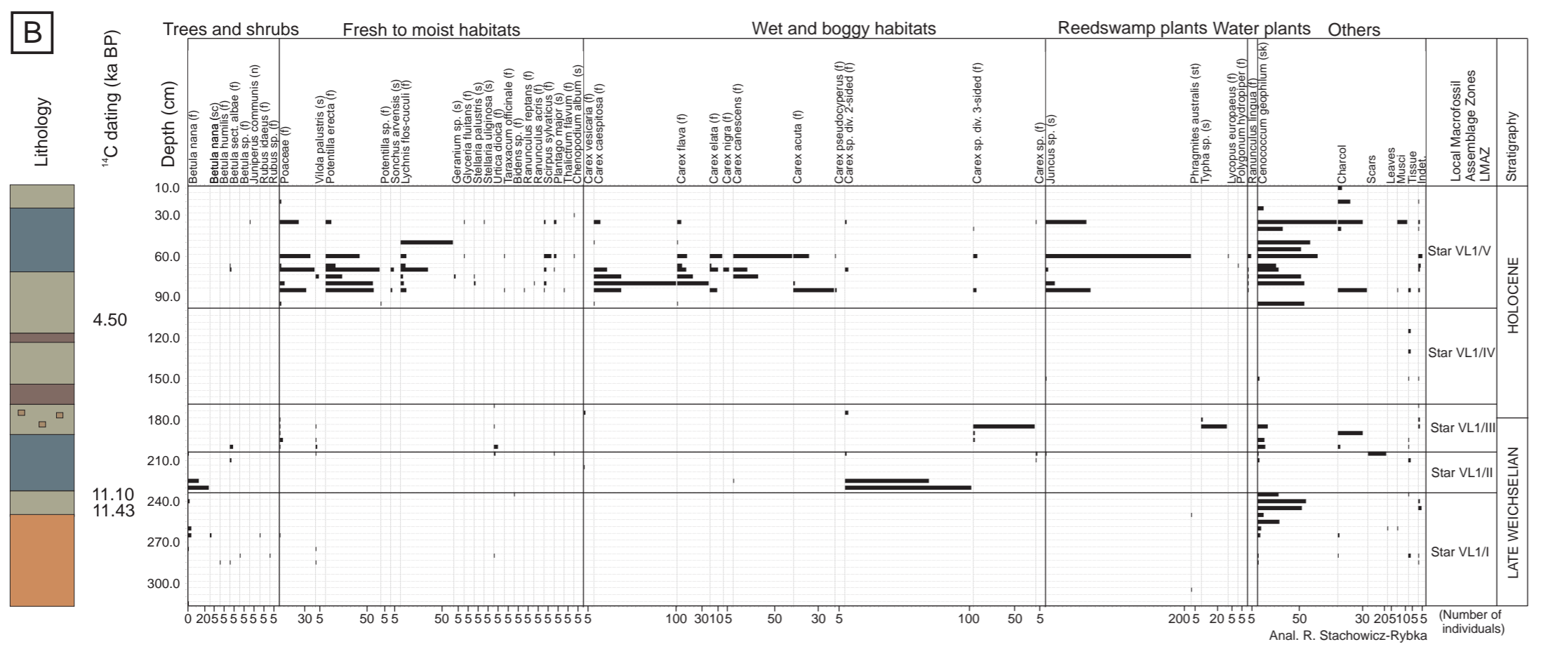
Fig. 3. Plant macrofossil diagram from from (A) borehole No. 22, and (B) outcrop VL-1
