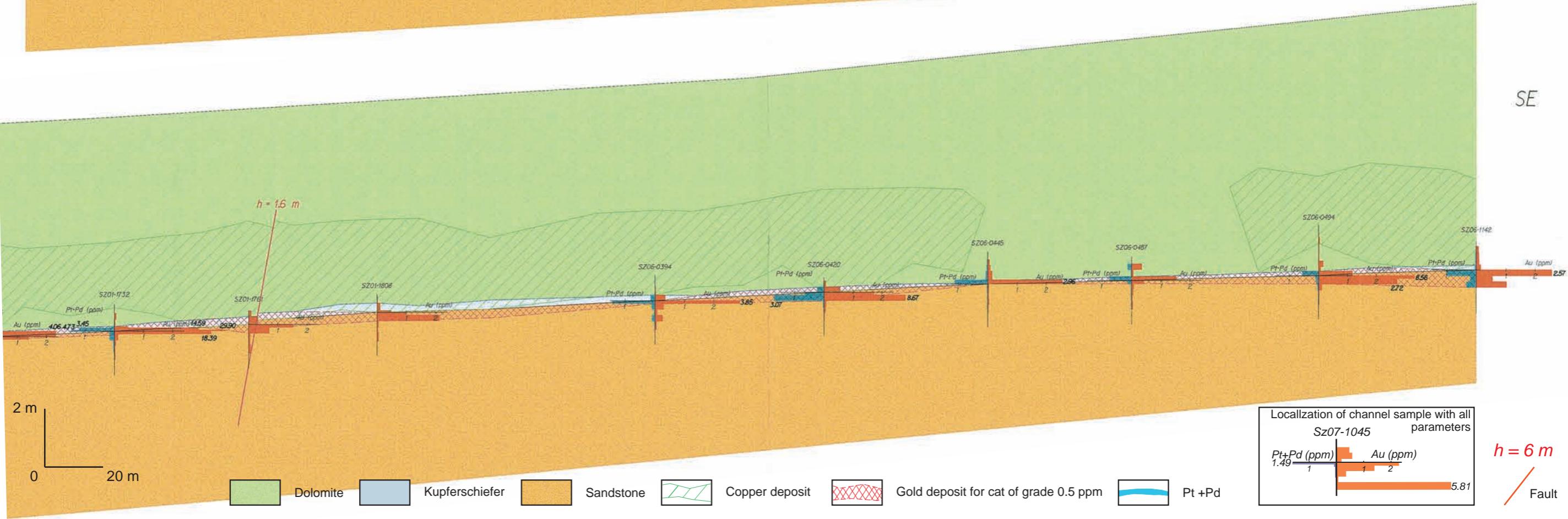
Fig. 82. Cross section P2r along mining work K-57W, Polkowice Mine, East Field
