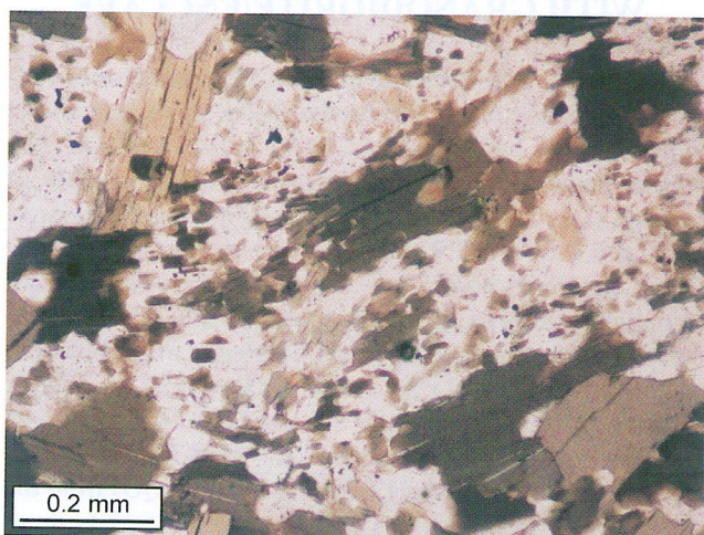
Fig. 5. Intergrowth of biotites flakes in sericitic pseudomorphs after cordierite in dark micaceous enclave, borehole DB-5, depth 1370.0 m. Plane-polarized light
