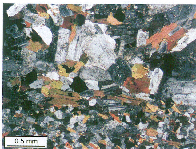
Fig. 9. Plagioclase plates and biotite flakes arranged parallel to the boundary of dark micaceous enclave and granodiorite from Będowska Valley, borehole DB-5, depth 1370.0 m. Crossed polars
