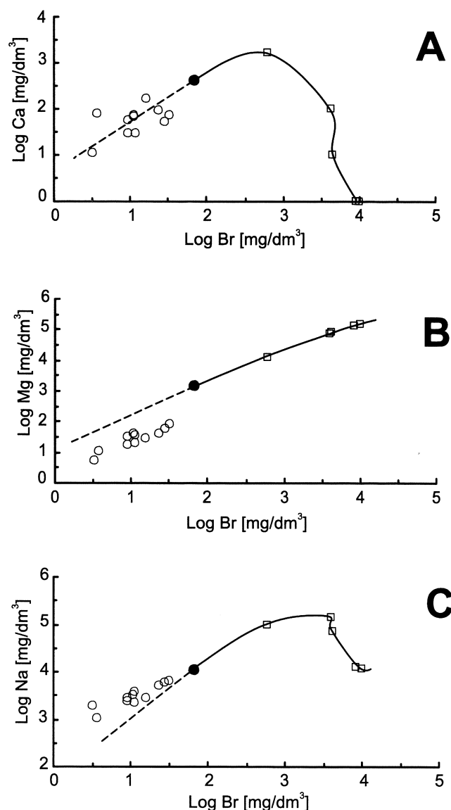
Fig. 7. Plots: A – log Ca vs log Br, B – log Mg vs log Br, C – log Na vs log Br, for Iwonicz anticline mineralized waters (open circles); seawater evaporation trajectories (open squares) for reference
