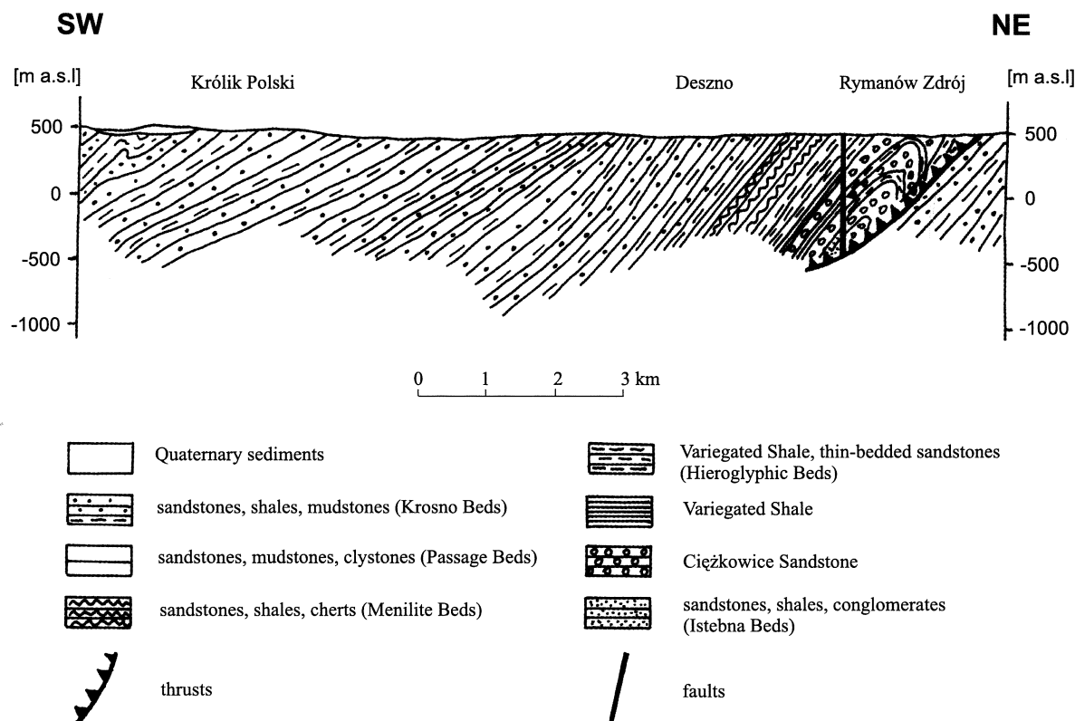
Fig. 2. Schematic geological cross section through the Iwonicz anticline at Rymanów. Modified by the author in relation to source version; source: Wdowiarz et al. , 1988
