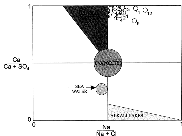
Fig. 4. Brine Differentiation Plot (BDP) (after Hounslow, 1995) and mineralized waters from Iwonicz anticline (open circles). Content of particular ions in mol/dm 3
