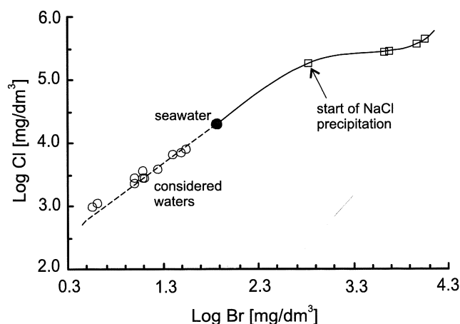
Fig. 5. Log Cl versus log Br for Iwonicz anticline mineralized waters with the seawater evaporation trajectory for reference; open circles – considered waters of Iwonicz anticline; open squares – particular stages of seawater evaporation
