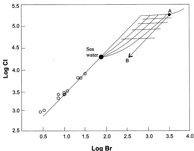
Fig. 6. Mineralized waters of Iwonicz anticline (open circles) and relationship between Cl and Br as a result of mixing NaCl-saturated brines with fresh water and with seawater. (Plot after Carpenter, (1978) modified by the author). For explanation see the text
