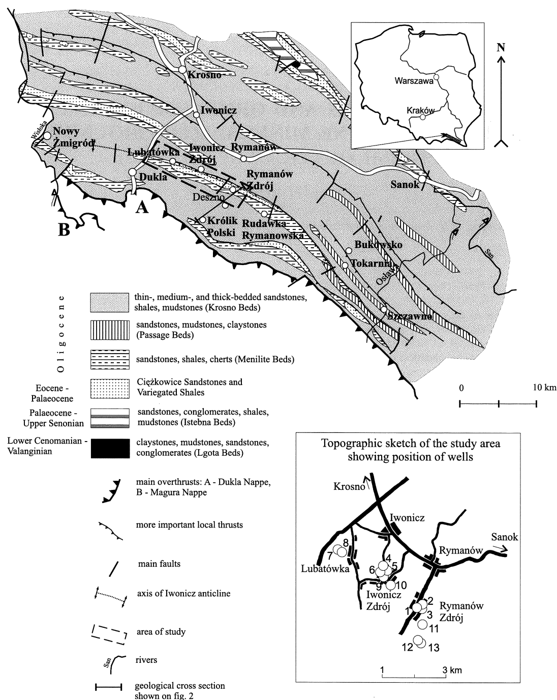
Fig. 1. The Iwonicz anticline and the position of considered mineralized groundwater intakes: 1 – spring Klaudia; 2 – spring Celestyna; 3 – spring Tytus; 4 – Elin 7; 5 – Emma; 6 – Zofia 6; 7 – Lubatówka 14; 8 – Lubatówka 12; 9 – Iwonicz 2; 10 – Klimkówka 27; 11 – Rymanów 2; 12 – Rymanów 5; 13 – Rymanów 6; Geological sketch was modified by the author in relation to source version; source: Poprawa & Nemcok (eds.), 1989
