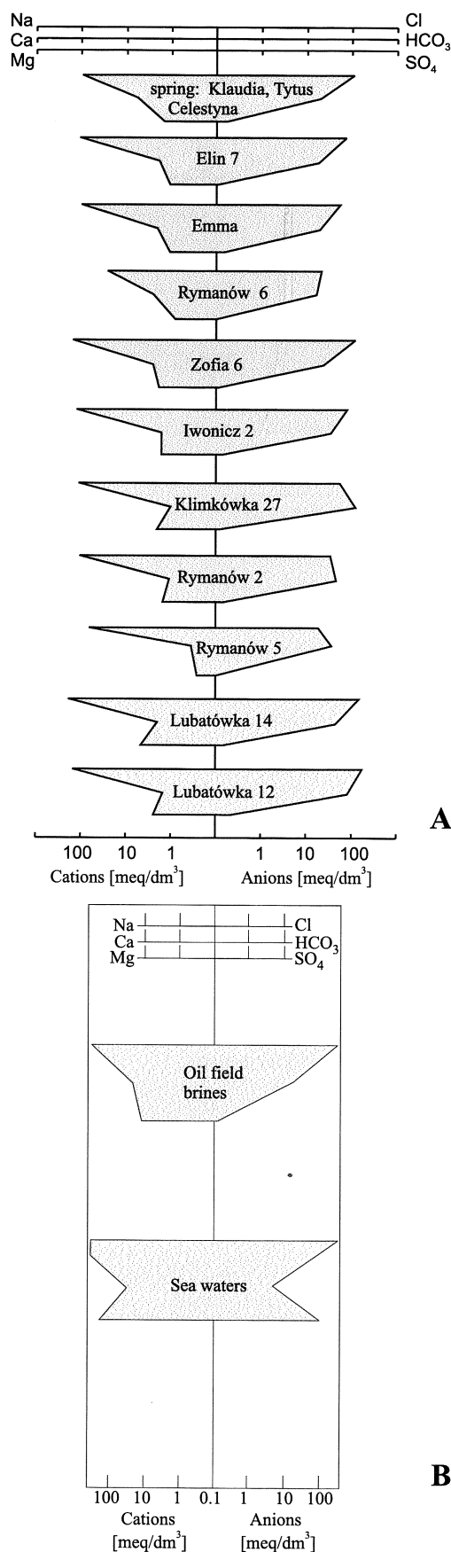
Fig. 3. Stiff diagrams for Iwonicz anticline mineralized groundwaters (A), and distinguished by Hounslow (1995) typical seawater and oil-field brines (B)
