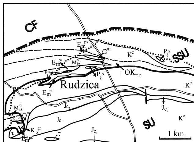
Fig. 2. Geological map of Rudzica area (after Nowak, 1966). τ – Teschenite sills; Kimmeridgian ?, Tithonian–Berriasian: Jc 1 – Lower Cieszyn Shales, Jc 2 – Cieszyn Limestones; Valanginian–Aptian: K c – Upper Cieszyn Shales, K o gr – Grodziszcz Sandstones; K m ps – variegated marls with intercalations of green marls (Turonian–Senonian); OK mlp – undivided deposits of Sub-Silesian Unit (Cretaceous–Tertiary); P i s – Upper Istebna Beds (Palaeocene); E m ps – variegated marls (Eocene); O m – Menilite Beds (Oligocene); M i o – clays, arenaceous clays with intercalations of clayey gravelstones (with fragments of flysch deposits) (Miocene). SU – Silesian Unit; SSU – Sub-Silesian Unit; CF – Carpathian Foredeep. Major tectonic boundaries: certain – drawn as continuous line; uncertain – discontinuous line. Area without data concerning pre-Quaternary deposits is marked by dotted line
