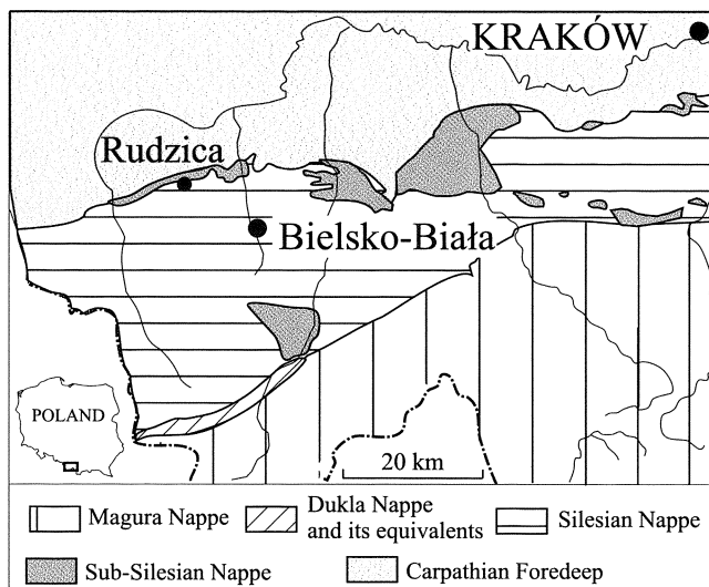
Fig. 1. Location and general geological sketch map (after Książkiewicz, 1977) of Rudzica area
