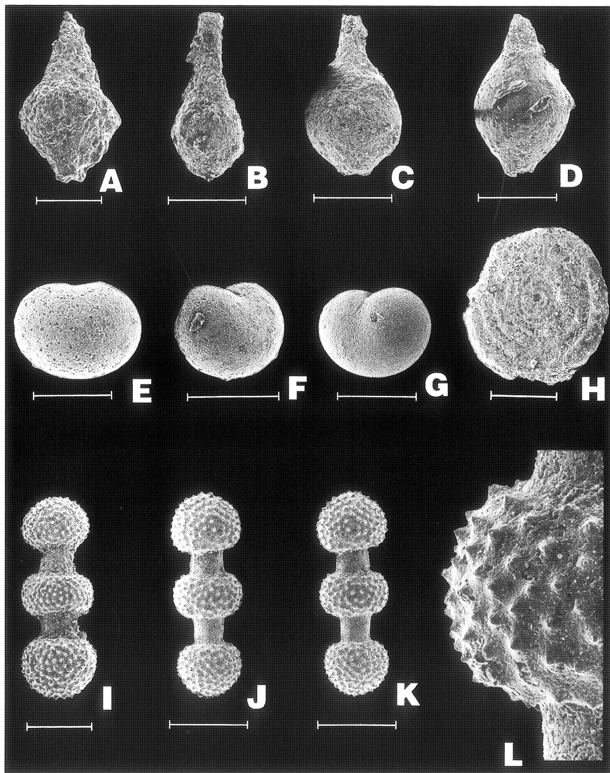
Fig. 10. SEM micrographs of Nassellaria, Foraminifera and sponge spicules. A-C. Syringocapsa vicetina (Squinabol); D. Syringocapsa sp.; E-G. Rhax ; H. Spirillina gracilis Terquem; I-L. Criccorhabd. Length of scale bar – 100 μm
