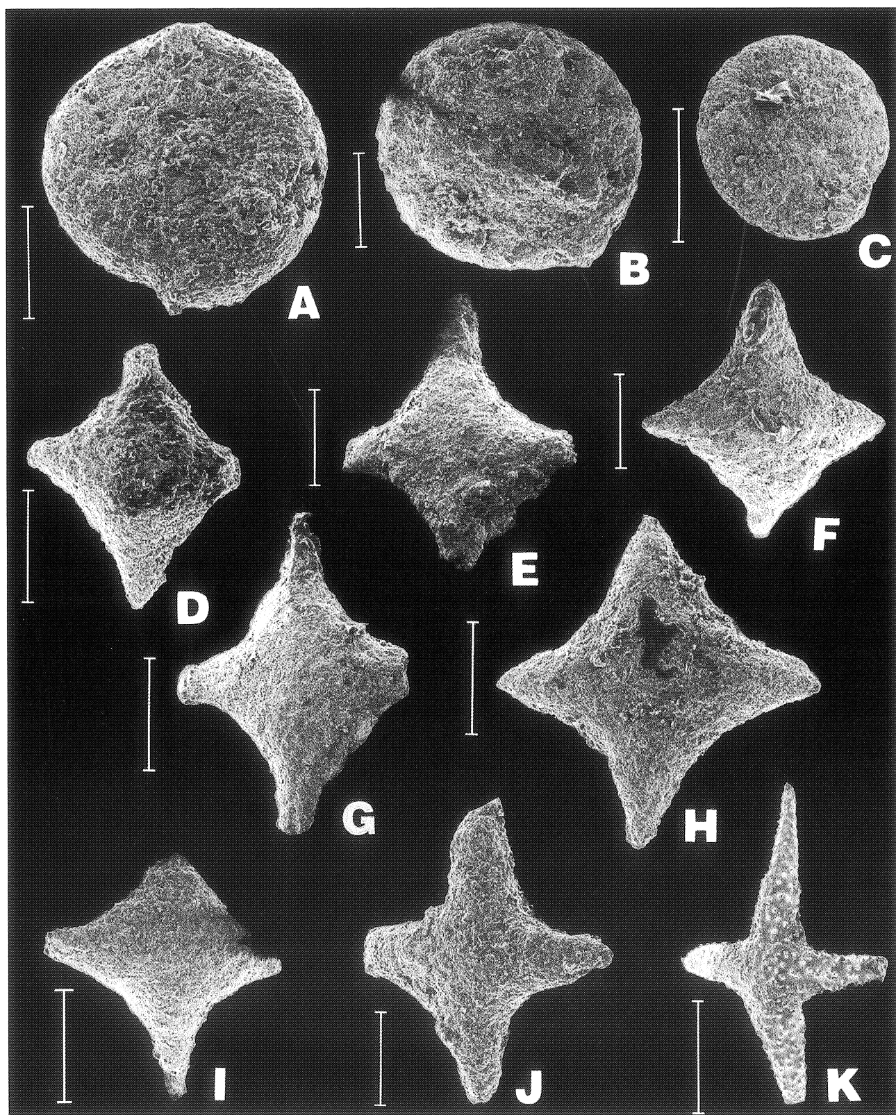
Fig. 7. SEM micrographs of Spumellaria. A-C. Orbiculiforma sp.; D-K. Crucella theokafensis Baumgartner. Length of scale bar – 100 µm
