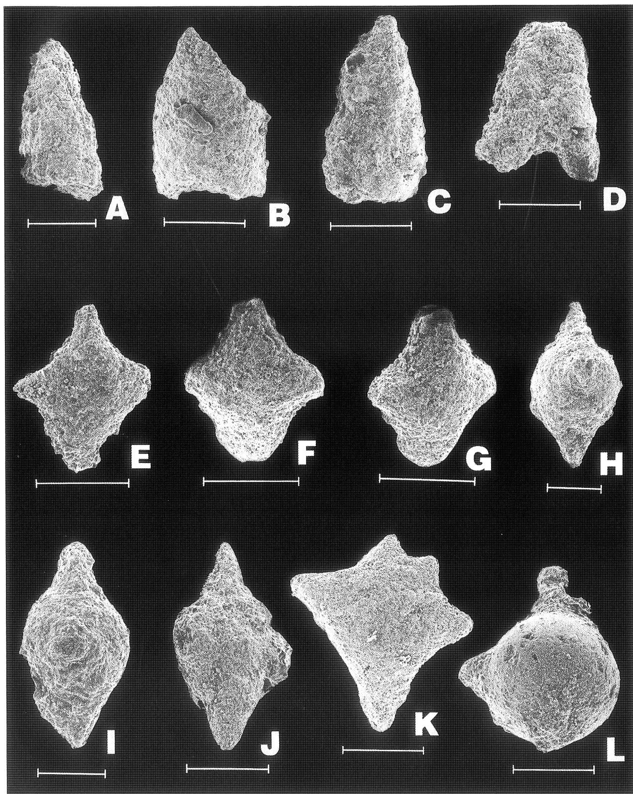
Fig. 9. SEM micrographs of Nassellaria. A-C. Hsuum sp.; D. Crolanium sp.; E-J. Dibolachras sp.; K. Podocapsa amphitreptera Foreman; L. Podocapsa sp. Length of scale bar – 100 \mu m
