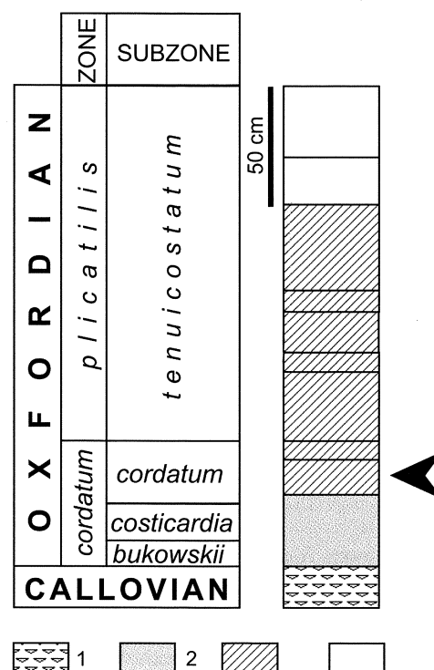
Fig. 2. Stratigraphic profile with ammonite zonal scheme (after Matyja & Tarkowski, 1981). Arrow marks position of radiolarian sample: 1 – stromatolite; 2 – marly limestone yellow and red; 3 – grey marly limestone with green and grey marls; 4 – grey marls and marly limestone
