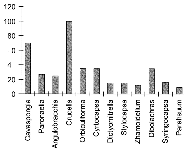
Fig. 3. Frequency (in number of specimens) of the radiolarian genera in the sample investigated
