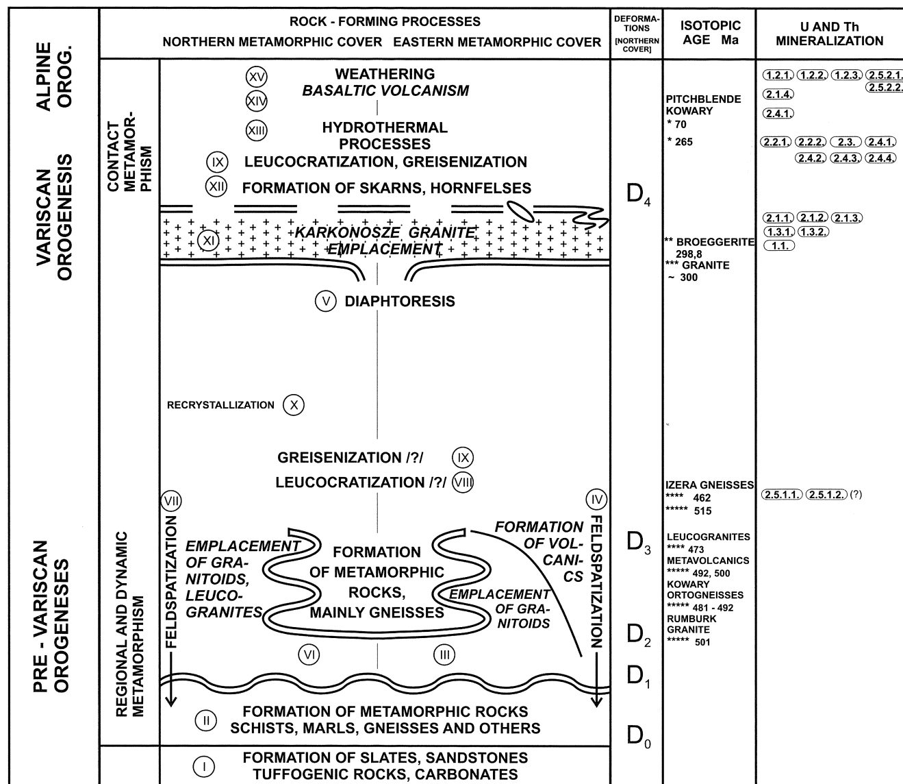
Fig. 2. Uranium and thorium mineralization related to the development of the Karkonosze Izer Block. Localities: 1.1. – Szklarska Poręba I, 1.2.1. – Maciejowa (Majewo), 1.2.2. – Bobrów, 1.2.3. – Trzcianko, 1.3.1. – Szklarska Poręba I, 1.3.2. – Karpacz, 2.1.1. – Szklarska Poręba III, 2.1.2. – Wołowa Góra near Kowary, 2.1.3. – Budniki near Kowary, 2.2.1. – Radoniów, 2.2.2. – Podgórze-Ruebezah Mine, 2.3. – Podgórze, 2.4.1. – Kowary, 2.4.2. – Ogorzelec-Victoria Mine, 2.4.3. – Miedzianka, 2.4.4. – Mnisków, 2.5.1.1. – Kopaniec-Mała Kamienica, 2.5.1.2. – Wojcieszyce, 2.5.2.1. – Kromnów, 2.5.2.2. – Czerniawa; * after Lis et al. (1971), ** after Kucha et al. (1986), *** approximate isotopic age after several authors, **** after Borkowska et al. (1980), ***** after Oliver et al. (1993), ***** after Korytowski et al. (1993)
