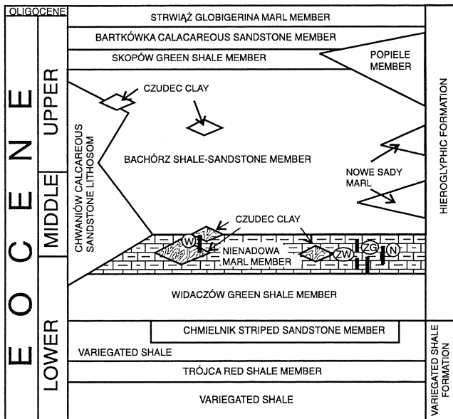
Fig. 2. Stratigraphic column of the Paleogene flysch deposits of the Skole Unit (after Rajchel, 1990). Studied sections: W – Wara; ZW – Zabratówka Wieś; ZG – Zabratówka Góra; N – Nienadowa
