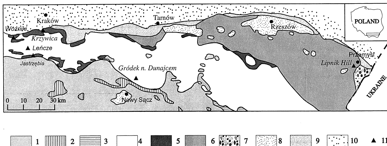
Fig. 1. Geologic sketch-map of part of the Polish Outer Carpathians (after Książkiewicz, 1972; partly changed): 1 – Magura Unit; 2 – Grybów Unit; 3 – Dukla Unit; 4 – Silesian Unit; 5 – Sub-Silesian Unit; 6 – Skole Unit; 7 – Stebnice Unit; 8 – Miocene deposits upon the Carpathians; 9 – Zgłobice Unit; 10 – Miocene deposits of the Carpathian Foredeep; 11 – location of exotics
