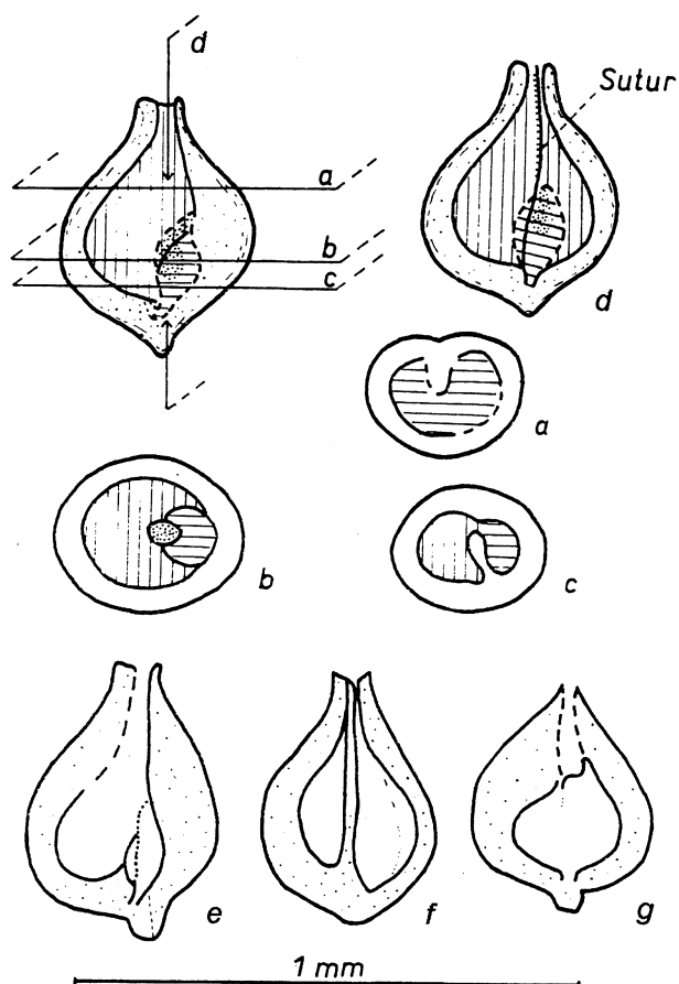
Fig. 1. Reconstruction of internal arrangement of Rothina silesica Hanzlíková; (a, b, c) the section planes through the test; (d) – section perpendicular to planes a, b, c; (e, f, g) – thin sections of real tests from Staříč NP 235 and NP 118 Boreholes (original figure after Hanzlíková, 1966)
