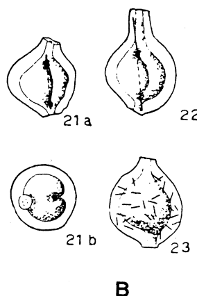
Fig. 2. Type figures of Hormosina ovulum crassa Geroch, after Geroch, 1966. A. Original fig. 6 (19, 21–26); Subsilesian Unit, ?Veřovice Shales, Sułkowice – Ubionka, (25 – holotype). B. Original fig. 7 (21–23); Silesian unit, Lhoty Formation, Straconka
