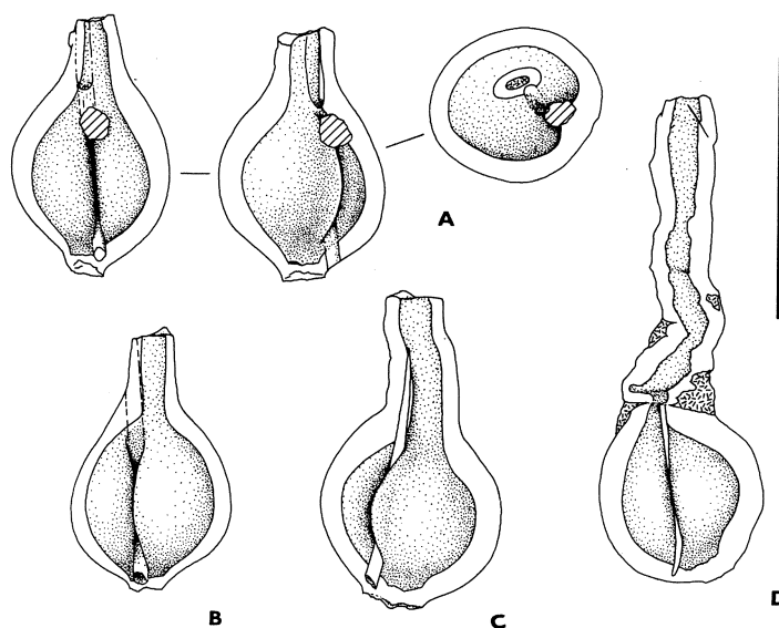
Fig. 3. Caudammina silesica (Hanzlíková). Specimens from the type collection of Hanzlíková: A. holotype, Staříč NP-177 (130.0–134.5 m); B. paratype, section G-15, south of Mořkov Village. C, D. Specimens from Staříč NP-118 Borehole (400 m). Total length of scale bar – 0.5 mm
