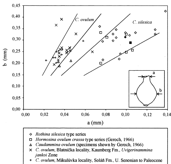
Fig. 6. Chamber/neck ( b/a ) diameter diagram. The holotypes of R. silesica and H. ovulum crassa marked by full black. A limit lines for Caudamina silesica and C. ovulum constructed after values given by Geroch (1959)
