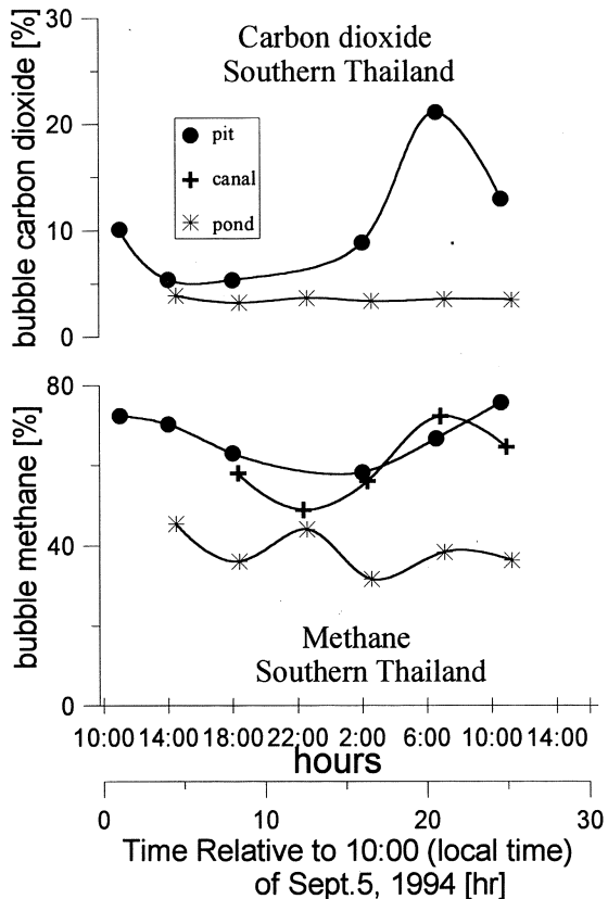
Fig. 4. Bubble CO 2 and CH 4 concentrations in sediment pore-gases of pit, canal and pond. See captions for Table 1 for details
