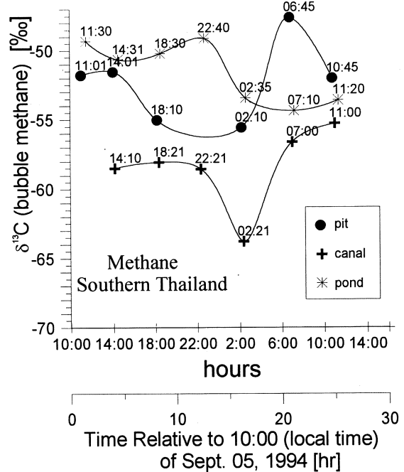
Fig. 6. Dial \delta^{13}\text{C} variations in bubble CH 4 from sediments in pit, canal and pond. See captions for Table 1 for details
