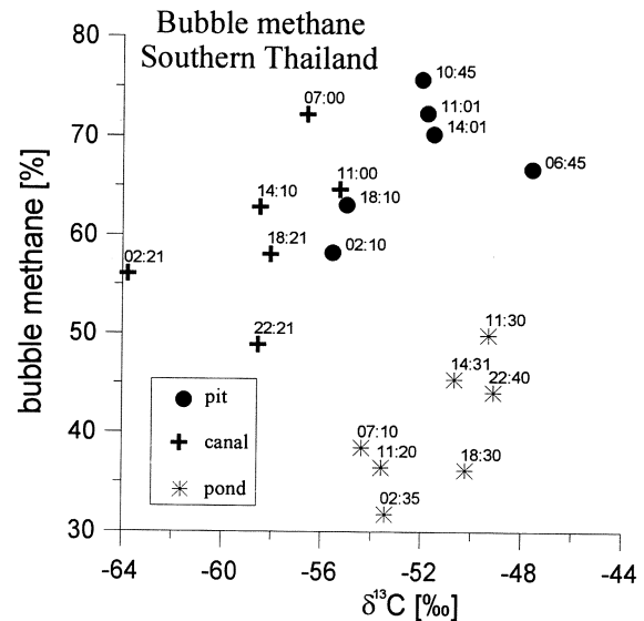
Fig. 8. Correlation of the bubble CH 4 and δ 13 CH 4 in pit, canal and pond. See captions for Table 1 for details
