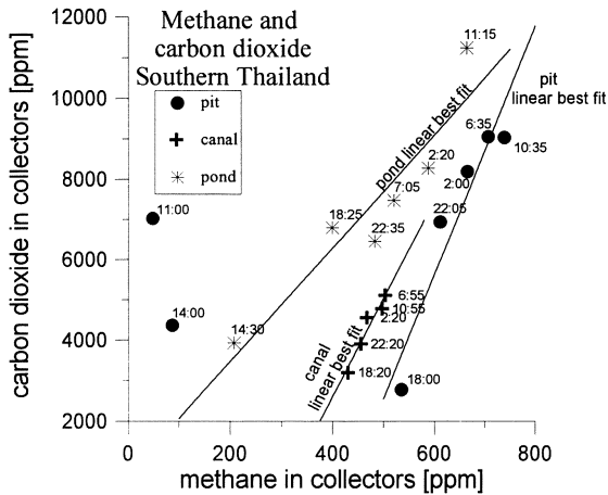
Fig. 3. Correlation of the CO 2 and CH 4 concentrations emitted from water surface of pit, canal and pond into floating chamber collector. See captions for Table 1 for details
