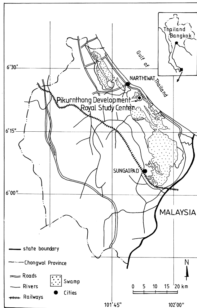
Fig. 1. Location of the study area (S Thailand)
