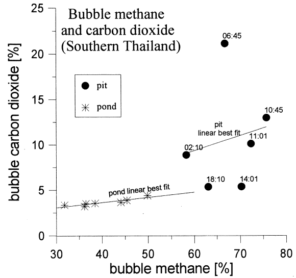
Fig. 5. Correlation of bubble CO 2 and CH 4 concentrations in sediment pore-gases in pit, canal and pond. See captions for Table 1 for details
