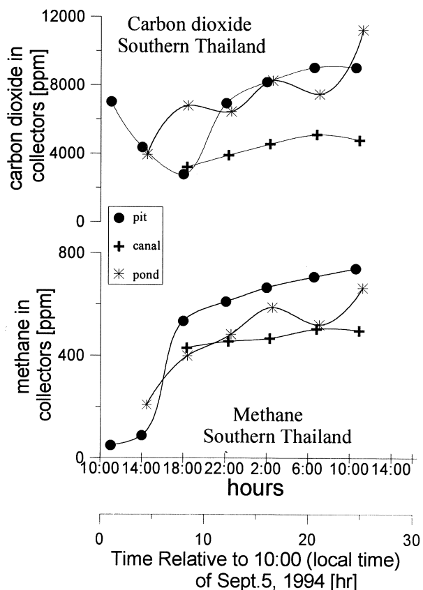
Fig. 2. CO 2 and CH 4 concentrations in chamber collector floating on water surface of pit, canal and pond. See captions for Table 1 for details
