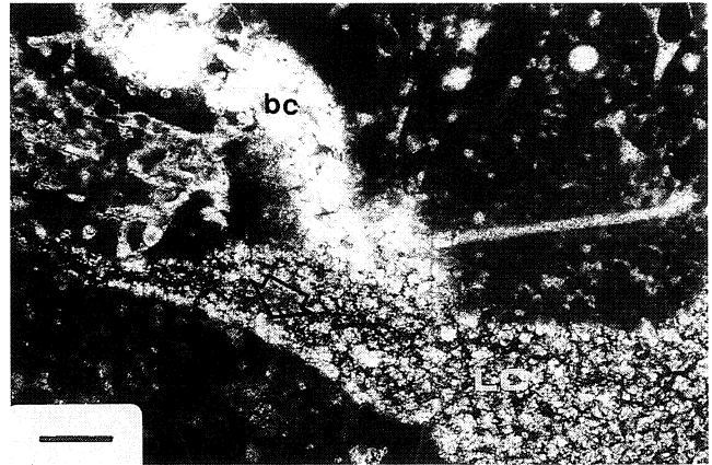
Fig. 7. The SIC in the Tubiphytes -reef at Zabierzów (the dark limestone). In the part of the SIC close to the roof, thin fractures branching from the cavity are filled with the transparent blocky cement (bc). The major part of the SIC is filled with the late cement (lc) containing numerous intercrystalline insertions. On the walls of the SIC are locally preserved relicts of the isopachous granular cement (arrow). Thin section, nicols parallel, scale bar 1 mm
