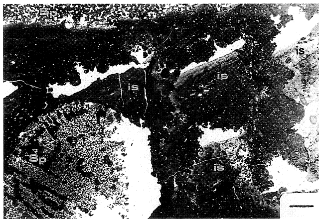
Fig. 3. The SCs in the cyanobacterial-sponge buildup at Młynka. Sp – calcified siliceous sponges. The upper parts of SCs are filled with cements. The internal sediment (is), filling the lower parts of the SCs, is clearly seen. Thin section, nicols parallel, scale bar 4 mm
