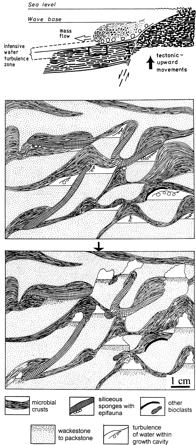
Fig. 9. Development of the SCs in a carbonate buildup with an initial stage of the rigid framework (partly after Matyszkiewicz, 1993). The cyanobacterial-sponge buildup developed at a moderate depth below wave base. The incipient laminar rigid framework was a delicate construction composed of cyanobacterial crusts and calcified siliceous sponges. Most of the spaces between the framework was filled with the soft carbonate mud, but part of the pore spaces and growth cavities was filled with sea water. Strong water turbulence, resulting from a mass flow induced by tectonic upward movements, caused washing out of the soft sediment around pore spaces and growth cavities and development a cavity network. This course of an internal erosion led to remodelling and the "upward migration" of cavities (cf. Wallace, 1987)
