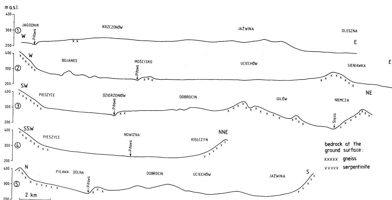
Fig. 3. Morphological profiles throughout the Dzierżoniów Basin (for location see Fig. 1)
