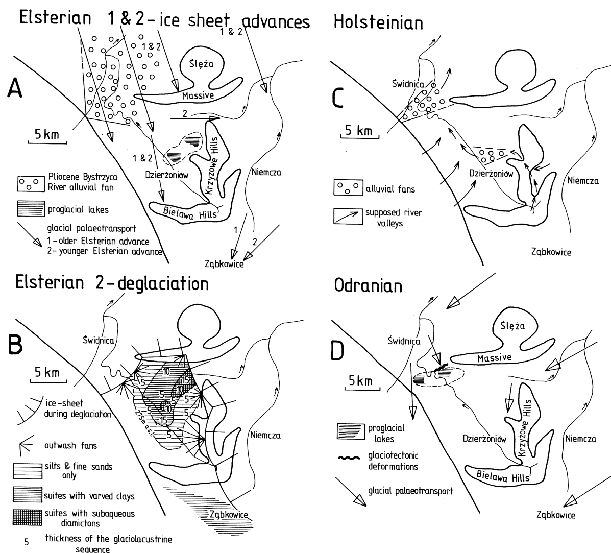
Fig. 19. Palaeogeographic interpretation of four case events (A-D) during the Middle Pleistocene in the Dzierżoniów Basin. Detailed discussion in the text
