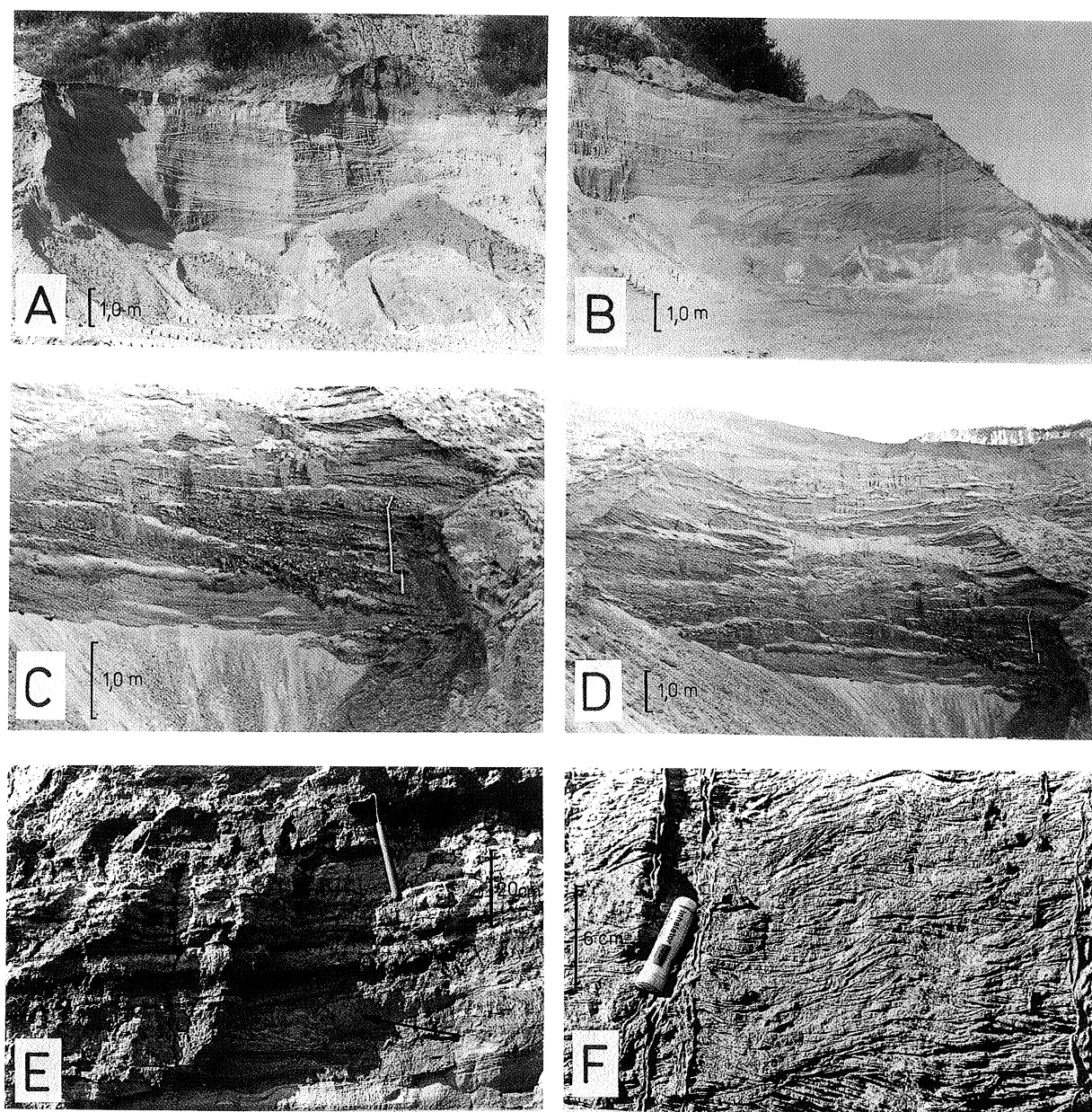
Fig. 10. Sediments at section Dobrocin 1K (A, B) and Dobrocin 1G (C, D) – note distinct cross-bedding and lithological changes in vertical profiles; E. Grodziszczce: varved clays with layers of deformed sands (arrow); F. Grodziszczce: deltaic fine sands with ripple cross-lamination
