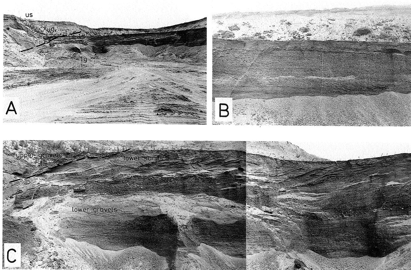
Fig. 9. Sediments of the section Dobrocin 1E. A. General overview with boundary between Lower and Upper Members; B. Lower gravels with visible cross-bedding and normal faulting; C. lower gravels and lower sands, note very distinct cross bedding and gradual transitions between lithological units (the section is 10 m high; northeast on the left)
