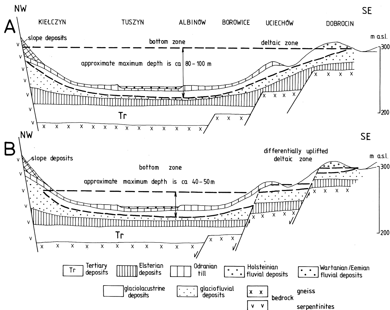
Fig. 21. Two alternative models of glaciolacustrine sedimentation during the deglaciation phase of the younger Elsterian stadial in the Dzierżoniów Basin. A. – with stable basement; B. – with inferred neotectonic movements (compare with fig. 19, discussion in the text)
