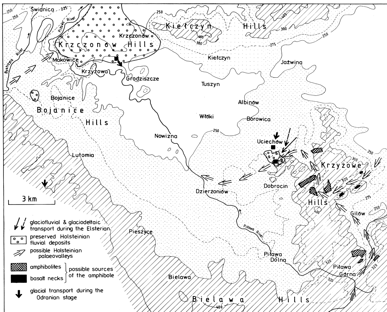
Fig. 20. Palaeoflows documented in fluvial and glacial sediments of Dobrocin, Uciechów and Grodziszcz quarries. Possible Holsteinian river courses are discussed in detail in the text. Altitude: white – below 250 m a.s.l., dotted – 250–300 m a.s.l., lined – above 300 m a.s.l.
