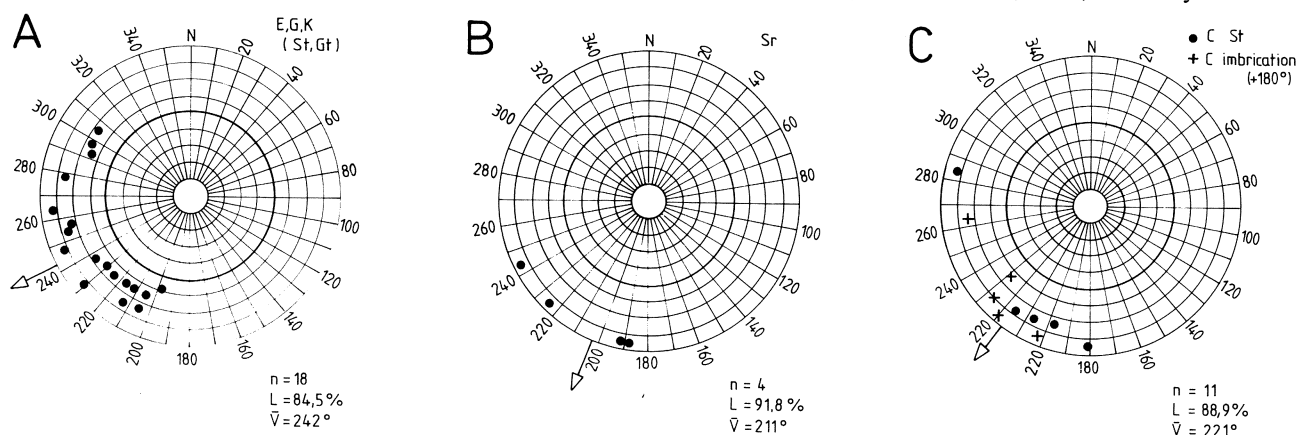
Fig. 14. Palaeoflow characteristics of the Dobrocin Formation: from Lower Member (A), glaciolacustrine silts and sands at section A (B) and Upper Member (C). Schmidt stereonet, southern hemisphere. n - number of measurements, L - vector amplitude, V - mean azimuth
