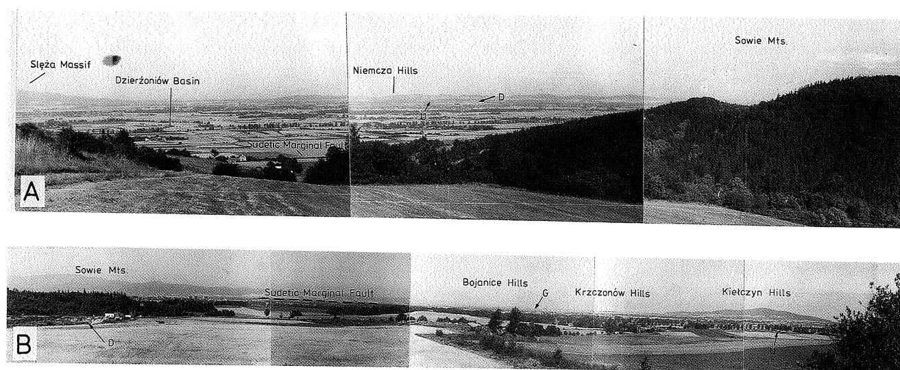
Fig. 2. General overview for the Dzierżoniów Basin: A. from Sowie Mountains to NE, on the left side is visible the "flat region" with alluvial veneers (northwest on the left); B. from Dobrocin quarry to the west, at the foreground hilly landscape between Dobrocin and Uciechów (southwest on the left); in both views: D – Dobrocin quarry, U – Uciechów quarry, G – Grodziszczę quarry
