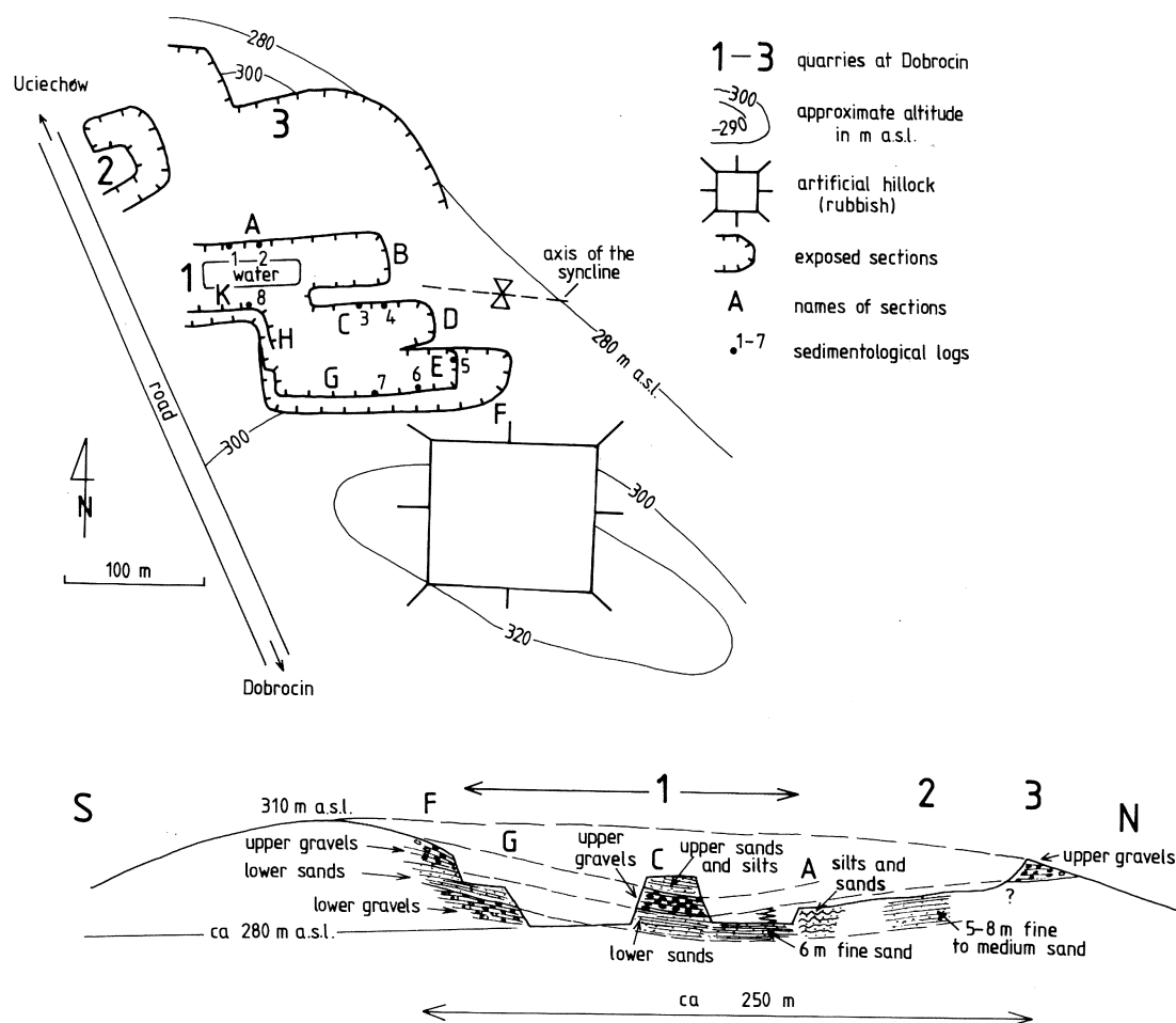
Fig. 4. A simplified map of Dobrocin quarry with location of sections and sedimentological logs (above) and cross section throughout quarries near Dobrocin with correlation of lithostratigraphic units (below)
