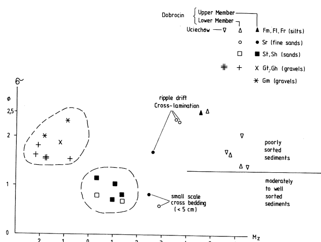
Fig. 13. Grain size characteristics of sediments at Dobrocin 1. Note similarities between deposits from different lithostratigraphic units. Lithofacial code after Miall (1977, 1978)
