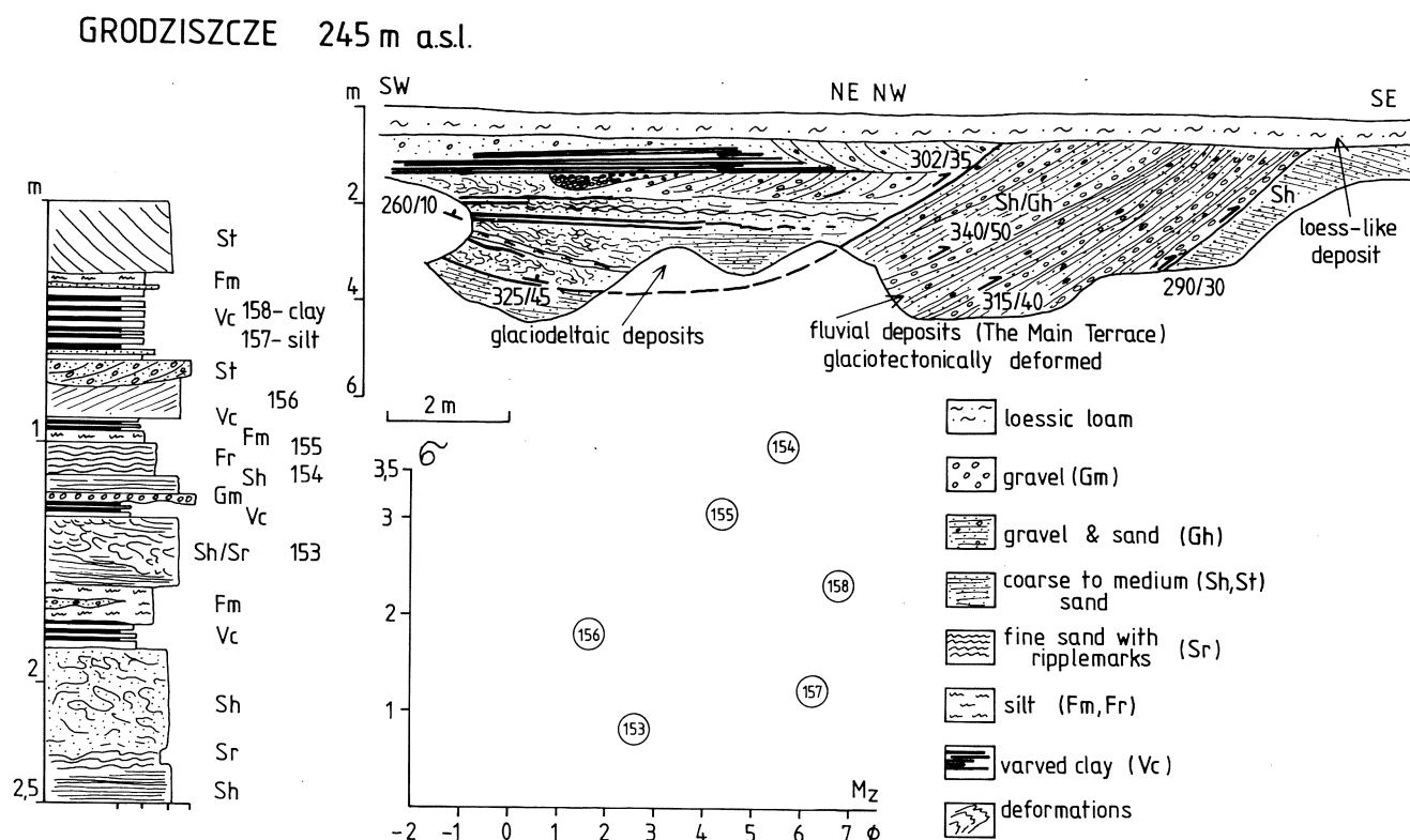
Fig. 16. Characteristics of glaciolacustrine sediments at Grodziszczce: general position at the section (upper right), sedimentological log and sampling (lower left) and grain size characteristics
