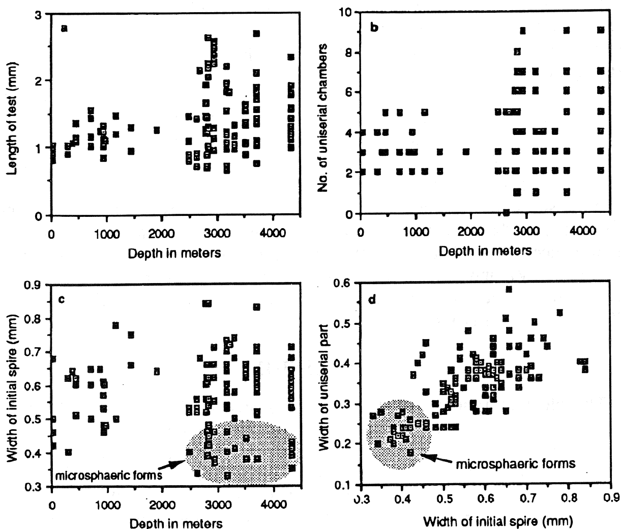
Fig. 4 Measured parameters of ALBATROSS specimens from the North Atlantic preserved in the Cushman Collection, arranged according to depth
