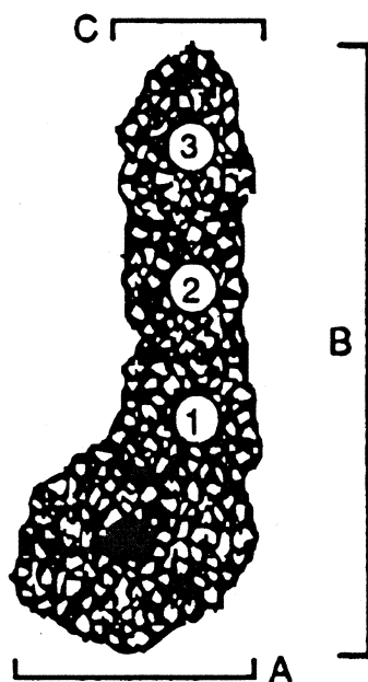
Fig. 2 Measured parameters in Ammobaculites agglutinans from the ALBATROSS Collection. A – maximum width across the initial spire, B – length of the test, C – maximum width of the uniserial portion, and the number of chambers in the uniserial part
