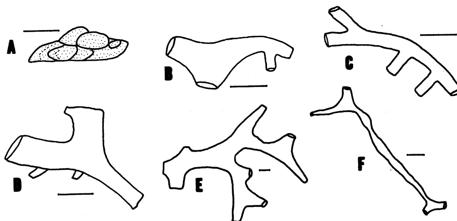
Fig. 2 Drawings of selected specimens. A – cross-section of sample with ?Thalassinoides ichnosp. showing “spreite”-like structure, Beloveža Beds (Lower – Middle Eocene), Uhryń, B – Thalassinoides ichnosp., Magura Formation (Upper Eocene), Lipnica Wielka, C – ?Ophiomorpha ichnosp., Beloveža Beds (?) (Lower – Middle Eocene), Rabka-Zaryte, D – Thalassinoides ichnosp., Magura Formation (Upper Eocene), Ponice, E – Thalassinoides ichnosp., Beloveža Beds (Lower – Middle Eocene), uncertain locality, Museum of Geology, Jagiellonian University, F – Thalassinoides ichnosp., Beloveža Beds (Lower – Middle Eocene), Roztoka. Scale bar = 2 cm
