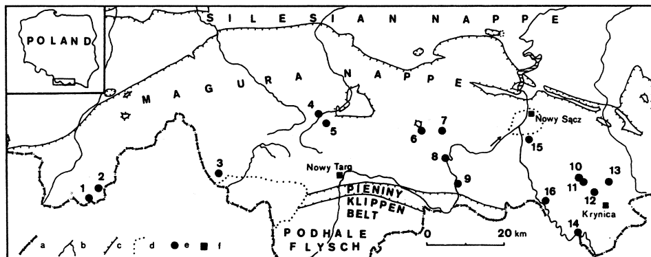
Fig. 1 Location of described sections; a – state boundary, b – main rivers and lakes, c – main overthrusts, d – outline of the Neogene post-tectonic cover, e – quoted localities (1 – Sobkówka, 2 – Glinka, 3 – Lipnica Wielka, 4 – Rabka-Zaryte, 5 – Ponice, 6 – Zasadne, 7 – Zbludza, 8 – Tylmanowa, 9 – Krościenko-Łąkcica, 10 – Łabowiec, 11 – Uhryń, 12 – Roztoka, 13 – Berest, 14 – Milik, 15 – Żeleźnikowa Wielka, 16 – Wierchomla Wielka), f – main towns
