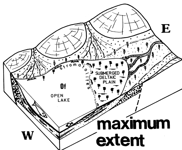
Fig. 11. Palaeogeographic reconstruction of the south-east part of the North Sudetic Basin during the phase of maximum extent of the Upper Anthracosia Lake. Of — offshore
