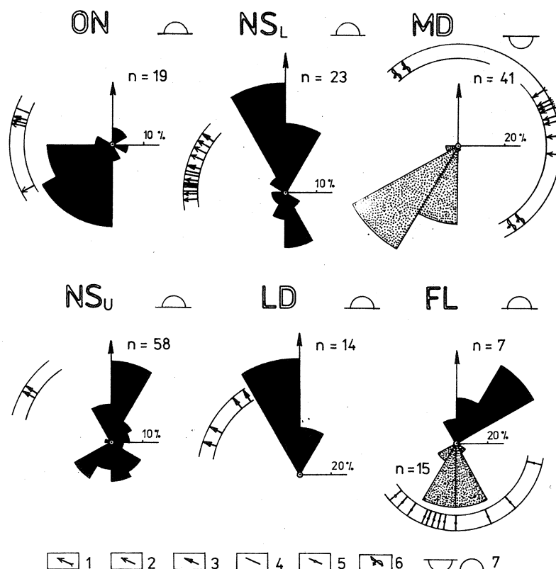
Fig. 4. Diagrams of directional sedimentary structures of the Upper Anthracosia Shale from the vicinity of Świerzawa. Rose diagrams: black — cross-lamination and bedding, stippled — pebble imbrication; facies: ON — onshore; NS — nearshore ( L — lower part; U — upper part); MD — mass-gravity deposits; LD — deltaic; FL — fluvial of the basal part of the Wielisławka Formation. Other palaeocurrent indicators: 1 — channel axes; 2 — trough cross-set axes; 3 — sole marks, current crescents; 4 — parting lineation; 5 — A-axis pebble orientation; 6 — slump fold axes and sense of a motion; 7 — upper- and lower-hemisphere projections
