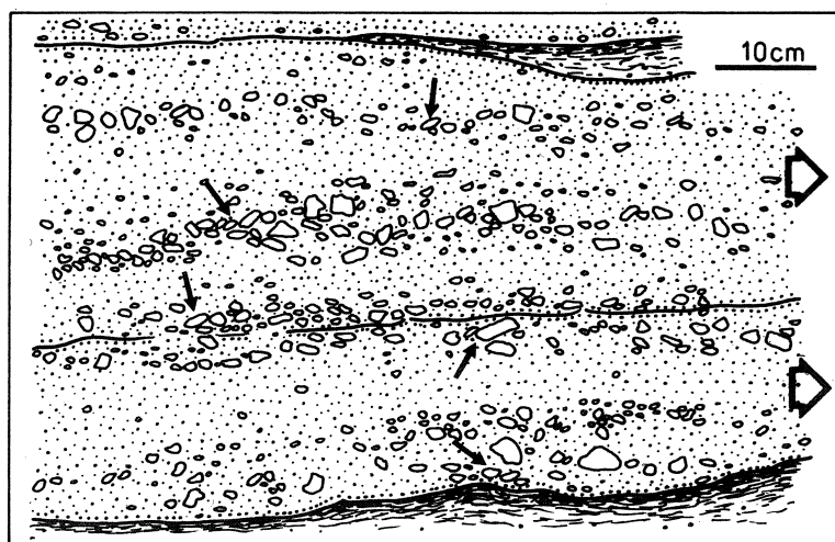
Fig. 8. Close-up view of the composite bed of amalgamated sandy conglomerate, mass-gravity facies. Note imbricate pebbles (arrows) and pebble segregation into stripes. Section oblique to palaeotransport direction (large arrows), Stara Krašnica
