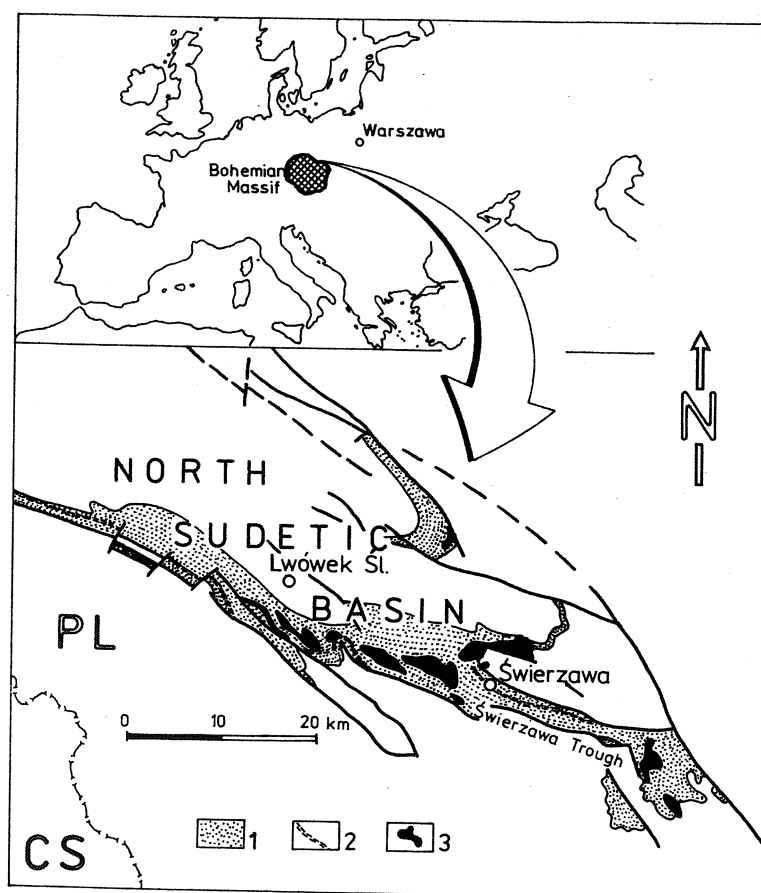
Fig. 1. Geological sketch-map of the North Sudetic Basin. 1 — Stephanian-Lower Permian sedimentary strata; 2 — Upper Anthracosia Shale; 3 — volcanogenic rocks
