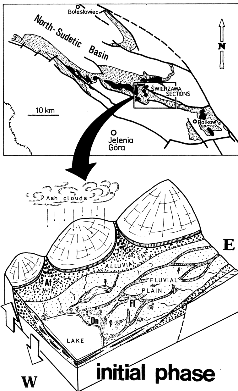
Fig. 9. Palaeogeographic reconstruction of the framed fragment of the North Sudetic Basin during the initial phase of the Upper Anthracosia Lake development. Af — alluvial fan; Fl — fluvial plain; On — onshore flat
