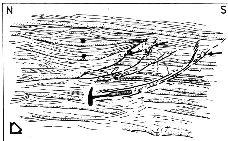
Fig. 3. Laminated sandstones and shales of the onshore facies, Stara Krašnica. Note listric surfaces of synsedimentary faults ( arrows ) and sets of trough cross bedding ( asterisks ). Section oblique to palaeotransport direction ( large arrow )
