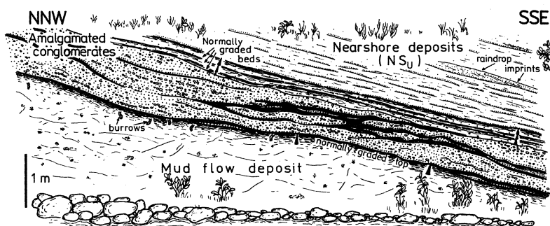
Fig. 7. Upper part of the sequence of mass-gravity deposits, Stara Krašnica
