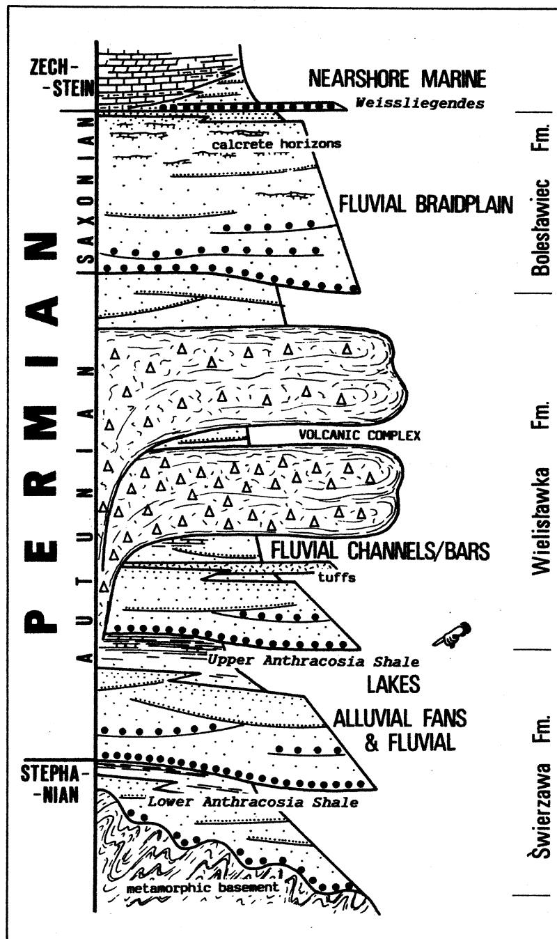
Fig. 2. Generalized lithostratigraphic column of the Stephanian-Lower Permian succession of the North Sudetic Basin
