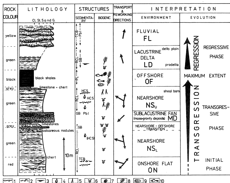
Fig. 5. Section of the lacustrine succession of the Upper Anthracosia Shale, Stara Krasnica: 1 — mud cracks; 2 — mud chips; 3 — sole marks; 4 — raindrop imprints; 5 — root casts; 6 — bioturbation; 7 — coprolites; 8 — plant remains; 9 — pelecypods; 10 — fish
