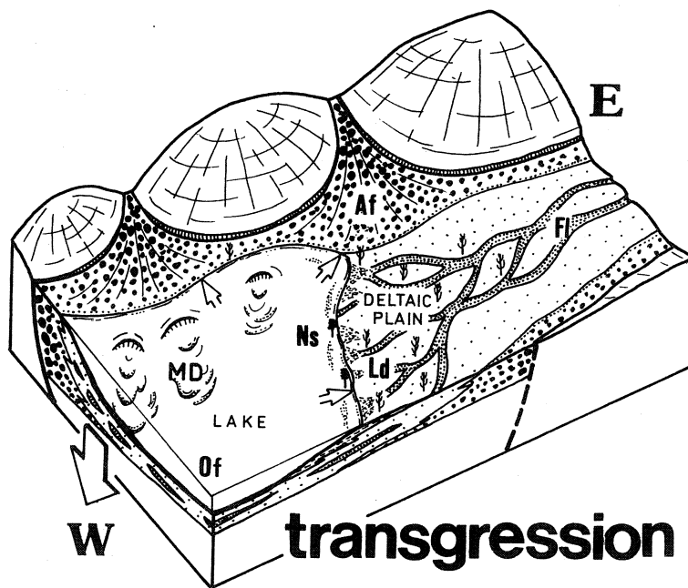
Fig. 10. Palaeogeographic reconstruction of the south-east part of the North Sudetic Basin during the transgressive phase of the Upper Anthracosia Lake development. Af — alluvial fan; Ns — nearshore; Ld — lacustrine delta; Of — offshore; MD — mass-displacement deposits
