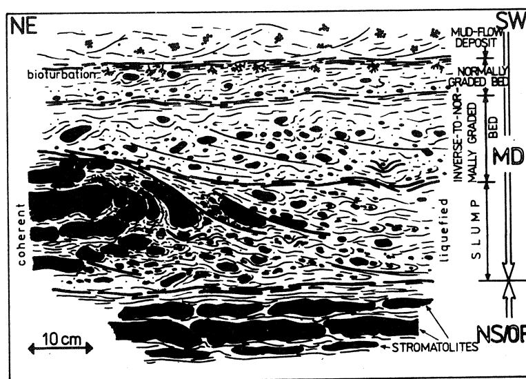
Fig. 6. Basal part of the sequence of mass-gravity deposits (MD) overlying stromatolitic limestones interbedded with mudstone of the nearshore-offshore transitional zone (NS/OF), Stara Krašnica
