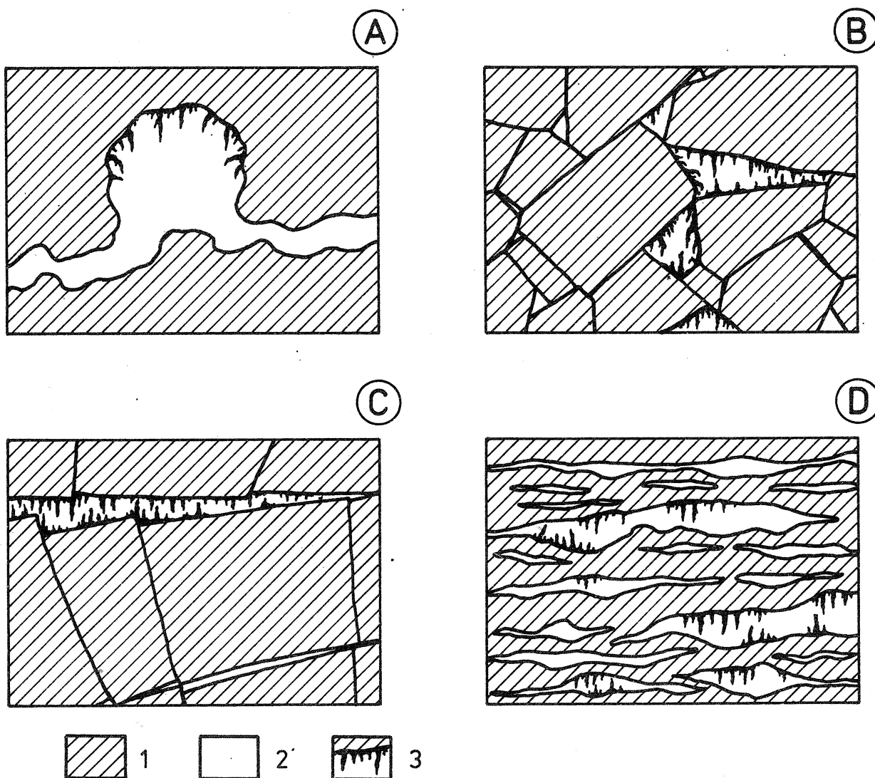
Fig. 2. Types of gas traps within Triassic carbonate formation: 1 — rock; 2 — void space; 3 — speleothems; A — part of original cave system; B — interfragmental spaces in breccia; C — crevices developed on bedding plane; D — open spaces within metasomatic sphalerite ore
