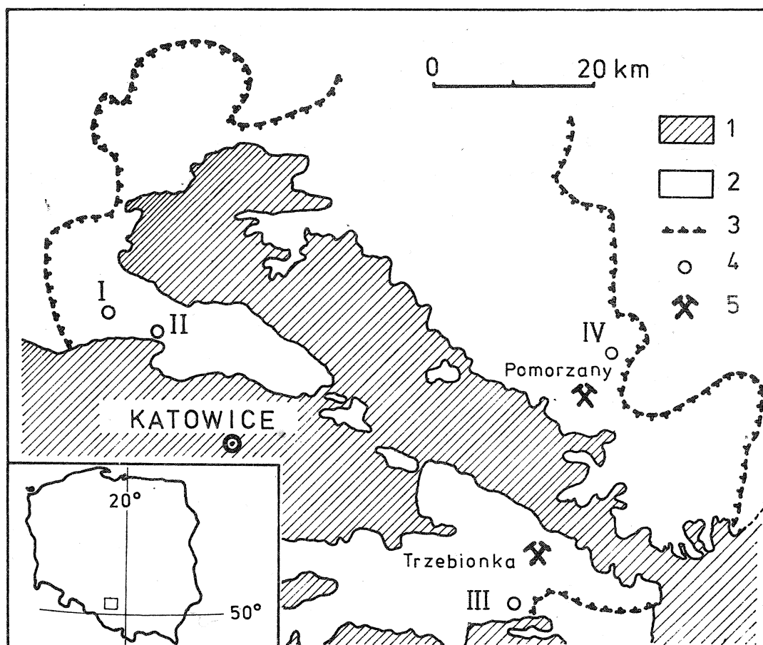
Fig. 1. Geological sketch of Upper-Silesian Zn-Pb ore district (without Jurassic and Cainozoic): 1 – Paleozoic (Upper Carboniferous and Permian); 2 – Triassic; 3 – boundary of ore district; 4 – localities of speleothems according to: I – Stappenbeck (1928), II – Wernicke (1930), III – Bartonec (1906), IV – Kuźniar (1925); 5 – localities of present investigations
