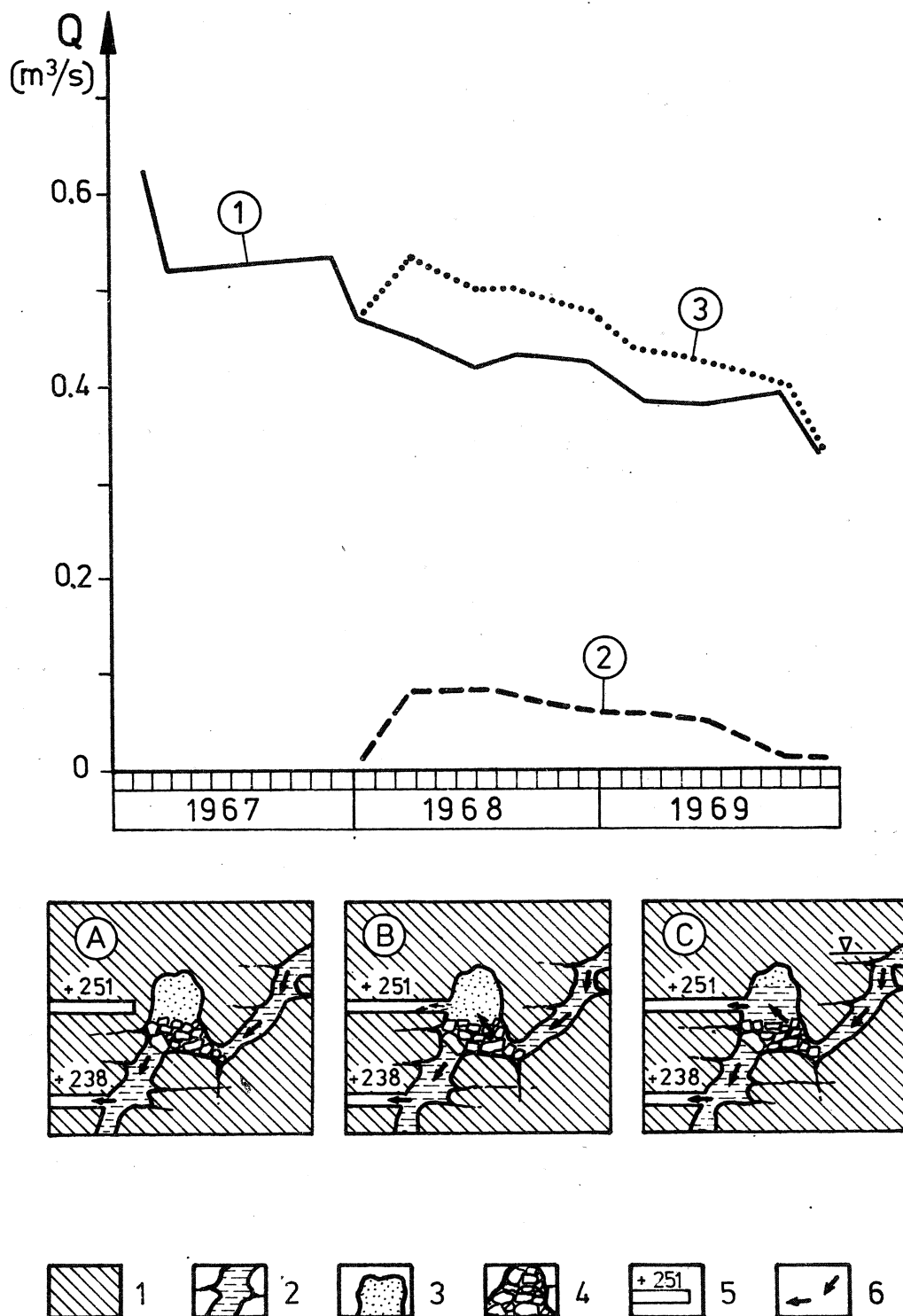
Fig. 5. Diagram of water output on level 238 (line 1), level 251 (line 2) and total (line 3). Interpretation of gas inflow: (A) — situation before digging up gas trap; B — gas inflow; C — water inflow. 1 — carbonate rocks; 2 — caves filled with water; 3 — caves filled with gas; 4 — caves filled with rock debris; 5 — mine gallery (with level designation); 6 — direction of water flow
