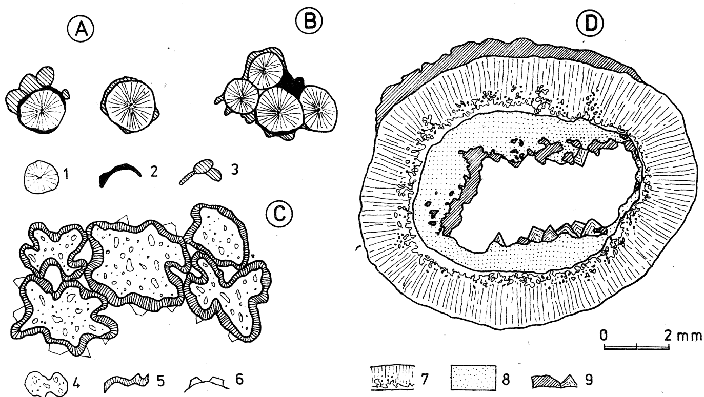
Fig. 3. Transversal sections of "stalactites": single (A) and aggregated (B) fine-crystalline marcasite forms, aggregate of sphalerite ones (C) and coarse-crystalline stalactite (D). 1 – marcasite rod; 2 – golden-coloured marcasite crusts; 3 – white marcasite crusts; 4 – porous sphalerite core; 5 – sphalerite crust; 6 – galena crystals; 7 – coarse-crystalline speleothem wall: dendritic carbonate layer covered with radially elongated sphalerite crystals; 8 – carbonate filling; 9 – crusts and druses of sphalerite and dolomite
