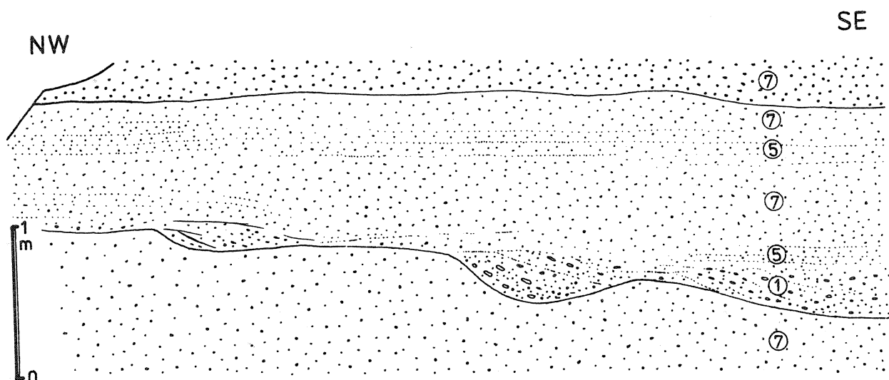
Fig. 8. Field sketch of composite pebbly sandstone bed (group PS) at the Skamieniałe Miasto protected site, near, Cieżkowice; Locality No. 7 in Fig. 1. Numbers refer to structural divisions explained in Table 2. The middle bed shows isolated trough cross-sets followed up by essentially homogeneous sandstone bearing two crude intervals with plane fine-sand laminae
