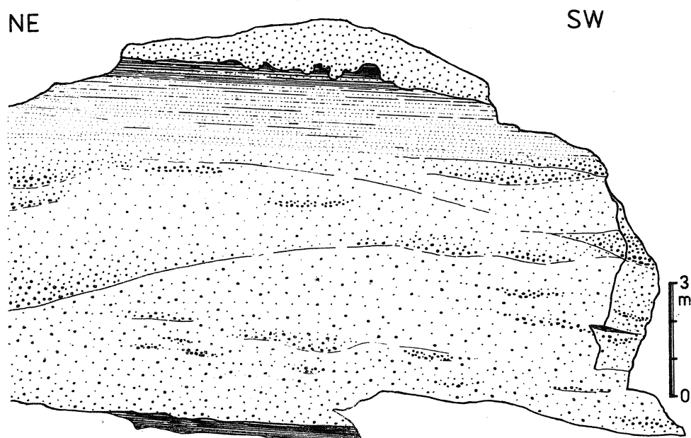
Fig. 15. Field example of composite bed showing extremely complex internal organization; quarry at Kaśna. Locality No. 7 in Fig. 1. Some conglomeratic lenses show trough cross-stratification. Topmost part of bed exhibits unusually thick parallel-laminated division ( T_p ) enriched in coalified plant matter
