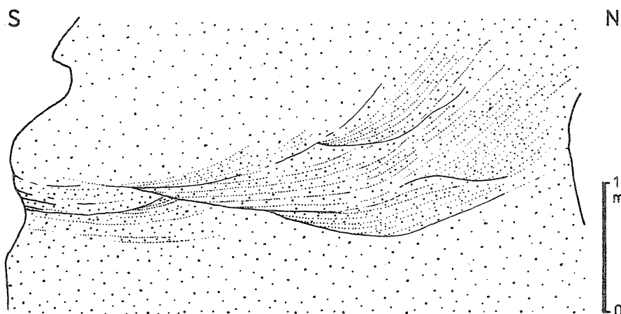
Fig. 10. Fragment of composite pebbly sandstone bed (group PS) exposed at Niedźwiedź Tor in the Skamieniełe Miasto protected site near Cieżkowice; Locality No. 7 in Fig. 1. Upper elementary bed shows trough cross-stratification picked out by fine-sand laminae and coarse-sand ones enriched with pebbles up to 8 mm in diameter. Note high angle of dip of cross-laminae in upper right of sketch. This cross-stratification resulted probably from shearing of freshly deposited load that began to freeze
