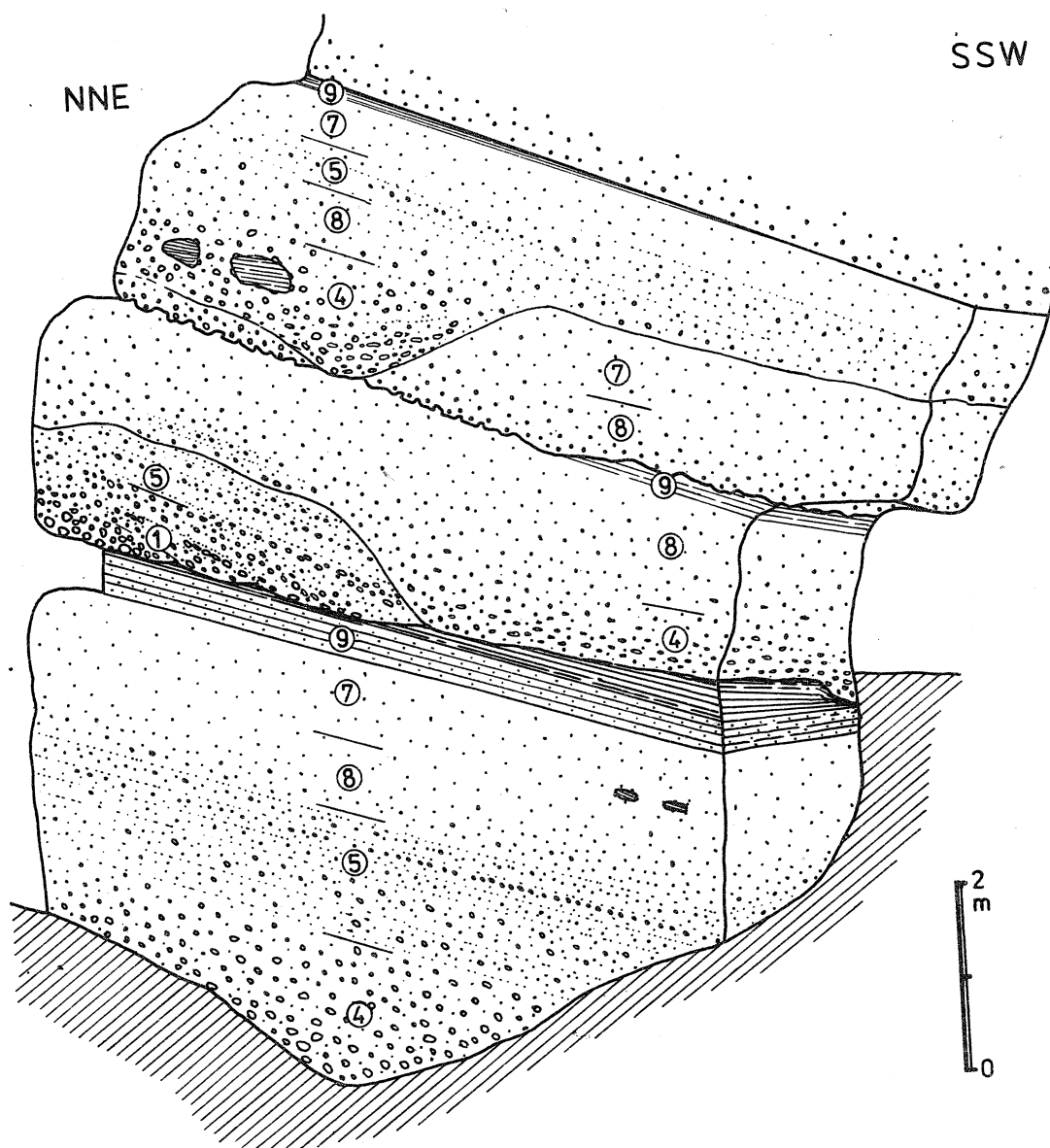
Fig. 5. Bedding and structures of conglomeratic and pebbly sandstone fluxoturbidite beds (groups CS and PS) at the Warownia Tor in the Skamieniale Miasto protected site near Cieżkowice; Locality No. 7 in Fig. 1; comp. Pls. I:2 and III:1. Numbers refer to structural divisions explained in Table 2. Simple bed is followed upwards by composite beds showing conspicuous channelling and rapid lateral changes in texture and structural development; note low-angle inclined parallel laminae in middle bed. These composite beds were probably deposited from surging flows
