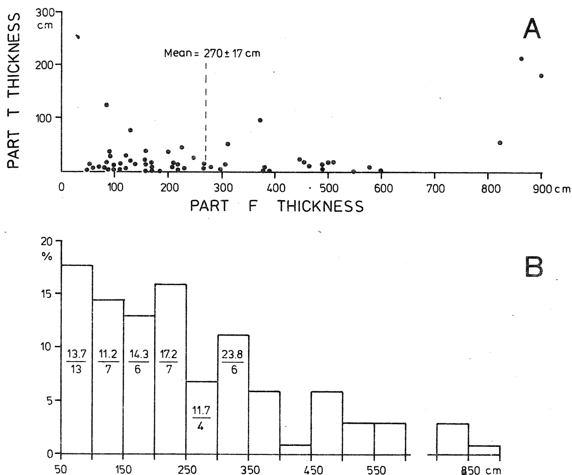
Fig. 4. Thickness characteristics of simple and pseudosimple fluxoturbidite beds (63 beds). (A) Plot of thickness of part F against thickness of overlying part T. (B) Thickness distribution of unit F; numbers given in histogram columns are mean thickness (cm) of part T (lower number) and mean percentage of part T within entire bed (upper number)
