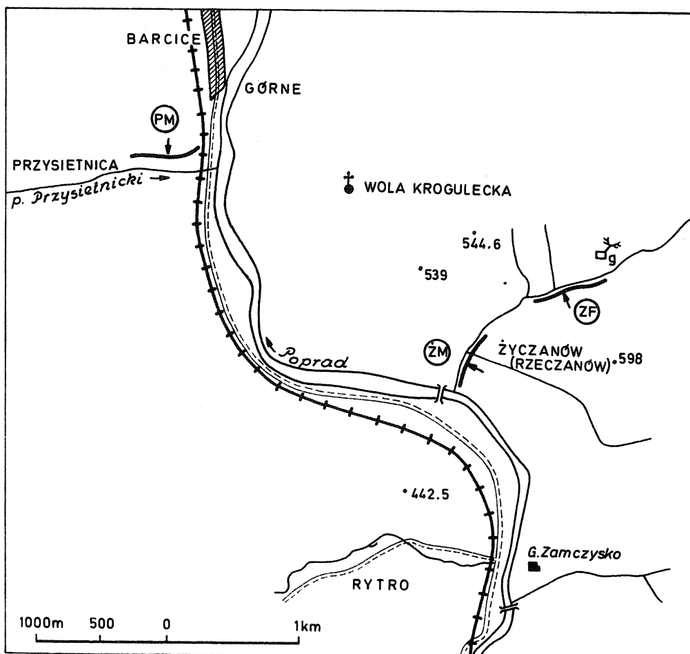
Fig. 3. Type and reference sections of the Piwniczna Sandstone Member (PM), Zarzecze Formation (ZF) and Życzanów Member (ŻM) in the Poprad Valley near Rytro
