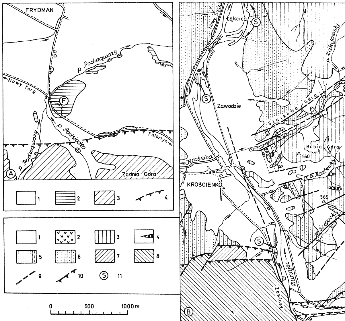
Fig. 6. A. Type section of the Frydman Formation (F) near Frydman. 1 – Quaternary cover; 2 – Frydman Formation; 3 – Grajcarek Unit of the Pieniny Klippen Belt; 4 – overthrust. B. Location of reference sections of the Szczawnica Formation in geological map of Krościenko (based on Birkenmajer, 1979). 1 – Quaternary cover; 2 – Miocene andesite intrusions; 3 – Magura Formation, Piwniczna Sandstone Member; 4 – Łącko marl intercalations; 5 – Zarzeczce Formation-type intercalations within the Piwniczna Sandstone Member and Zarzeczce Formation; 6 – Szczawnica Formation; 7 – Grajcarek Unit; 8 – Klippen Successions; 9 – main Tertiary faults; 10 – main Tertiary overthrusts; 11 – reference sections of the Szczawnica Formation
