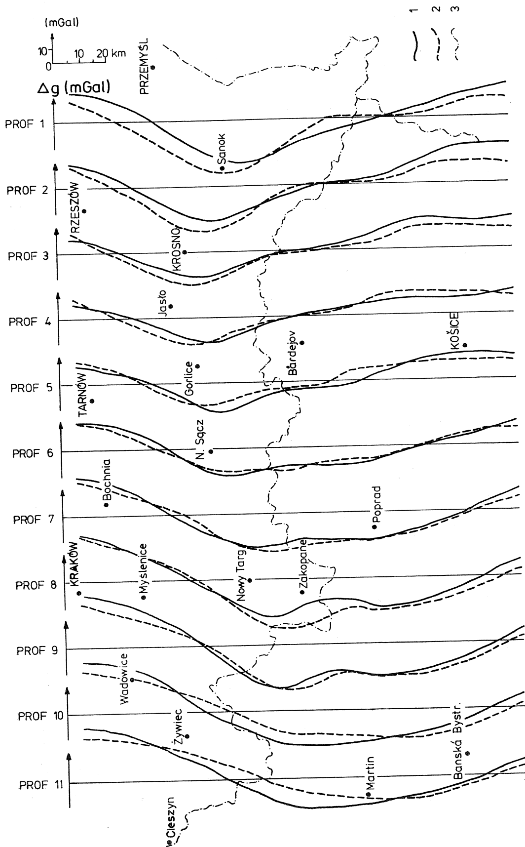
Fig. 11. Comparison of calculated gravity effect of three-dimensional model of crust and upper mantle with regional gravity anomalies calculated with Grif-fin's method for radius R = 5\sqrt{2} km. 1 — gravity effect of the model; 2 — regional anomaly; 3 — state boundary
