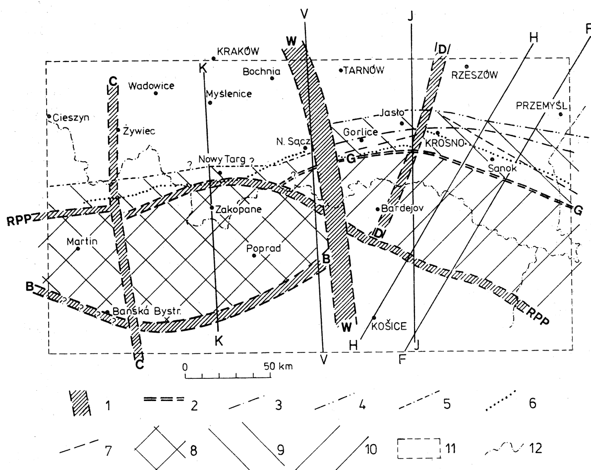
Fig. 8. Tectonic sketch-map showing main crustal elements in the Polish and Slovak Carpathians. 1 — fracture zones ( RPP — Peripienine fracture zone); 2 — G—G line — northern boundary of oceanic crustal fragment in northern plate; 3 — northern boundary of the Moho depression related to the lowered fragment of northern plate; 4 — northern boundary of “Conrad surface” depression related to the lowered fragment of northern plate; 5 — supposed extent of the lowered fragment in northern plate, west of W—W fracture zone; 6 — axis of gravity minimum; 7 — axis of depression in the basement of sedimentary rocks of density 2.63 \text{ g/cm}^3 (according to the model); 8 — area of thickened crust in southern plate; 9 — lowered fragment of northern plate; 10 — area of occurrence of oceanic crustal fragment in northern plate; 11 — boundaries of three-dimensional model; 12 — state boundary. Profile symbols as in Fig. 1
