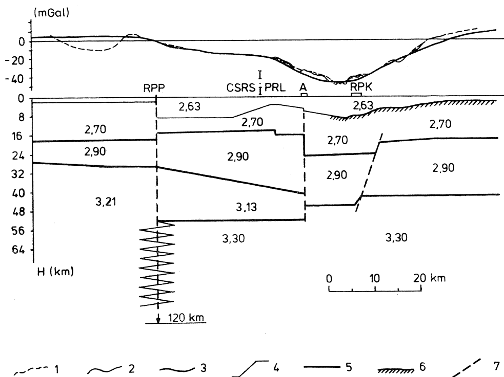
Fig. 3. Model of crust and upper mantle along Jaśliska—Mielec profile. Explanations in Fig. 2
