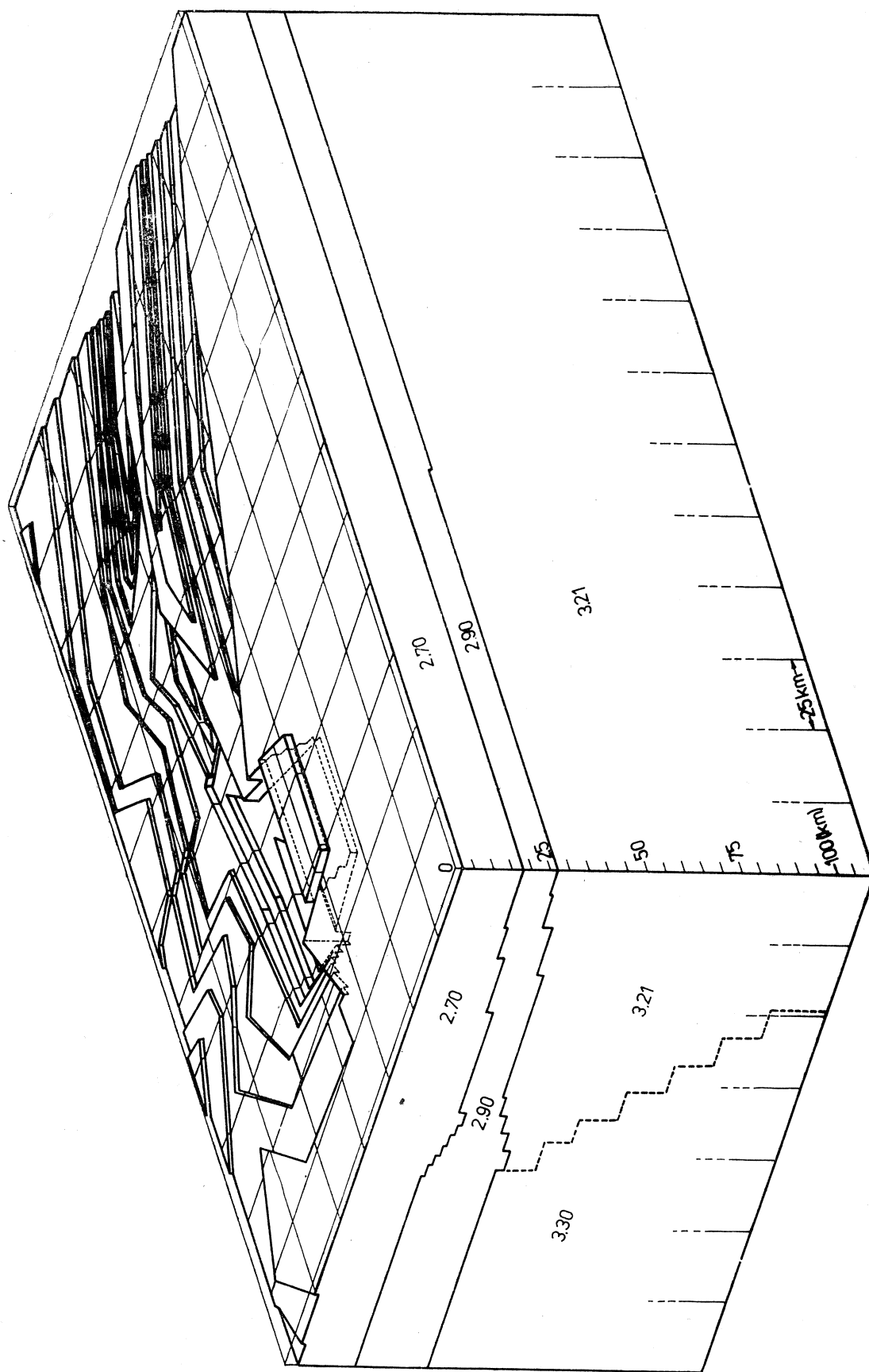
Fig. 7B. Model of the top of crystalline basement. Blockdiagram (view from SW)
