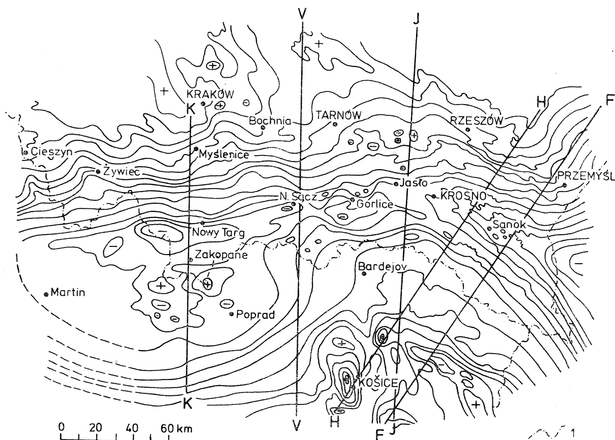
Fig. 1. Map of gravity anomaly after Jamrozik (1965) and Bednař et al. (1980). Contour distance 5 milligals. V—V — Vth International DSS Profile; F—F — Baligród—Radymno profile; H—H — Jaśliska—Błażowa profile; J—J — Jaśliska—Mielec profile; K—K — Kraków—Zakopane profile; I — state boundary
