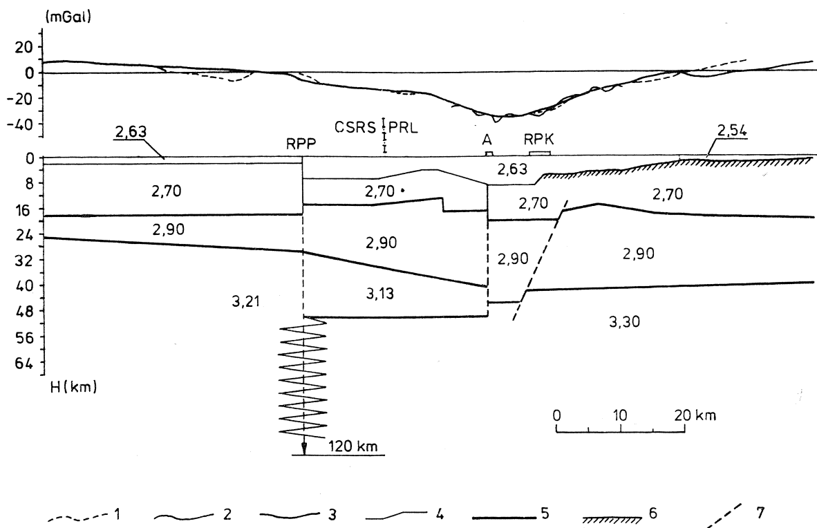
Fig. 2. Model of crust and upper mantle along Jaśliska—Błażowa profile. 1 — curve of observed \Delta g_B anomaly after regional map by Jamrozik (1965); 2 — curve of observed \Delta g_B anomaly after regional survey by Maryniak (1951); 3 — curve of gravity effect of the model; 4 — top of sedimentary rocks of density 2.7 g/cm 3 ; 5 — other density boundaries; 6 — top of crystalline basement after seismic refraction and magnetotelluric soundings; 7 — discontinuity (fracture?) zones in the crust; RPP — Peripienine fracture, RPK — Pericarpethian fracture. Zig-zag line is the graphic representation of horizontal density gradient in upper mantle
