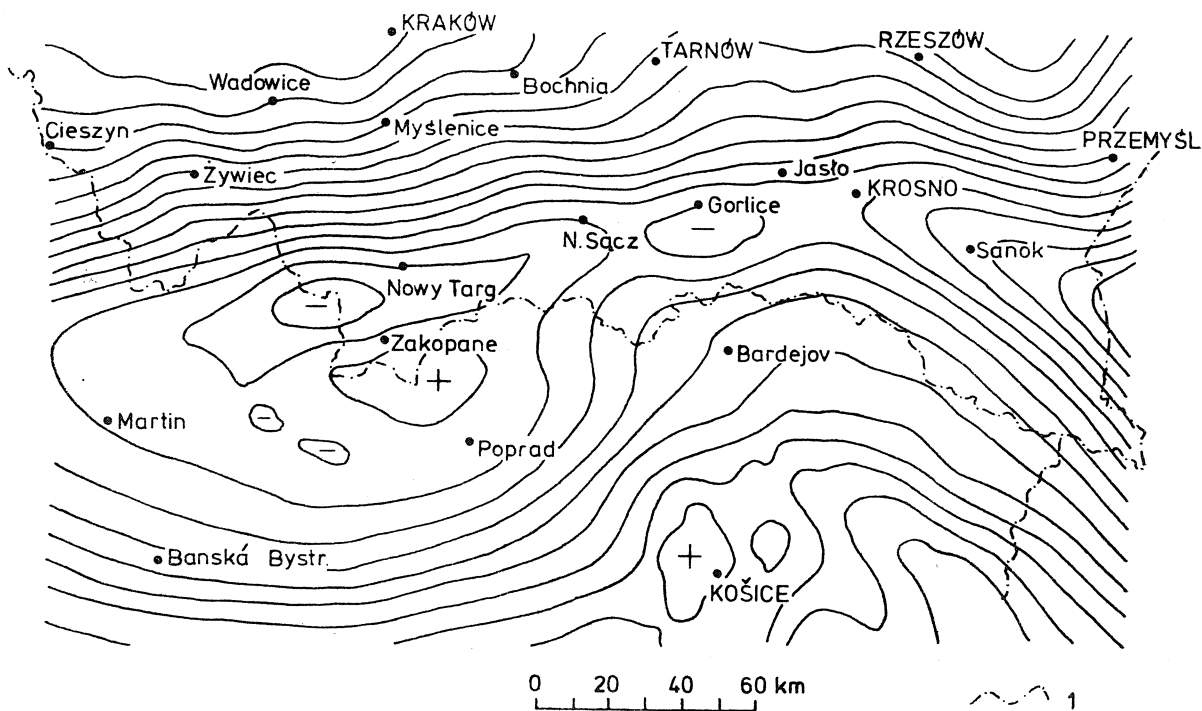
Fig. 10. Map of regional gravity anomalies calculated with Griffin's method for radius R = 5\sqrt{2} km. Contour distance — 5 milligals. 1 — state boundary
