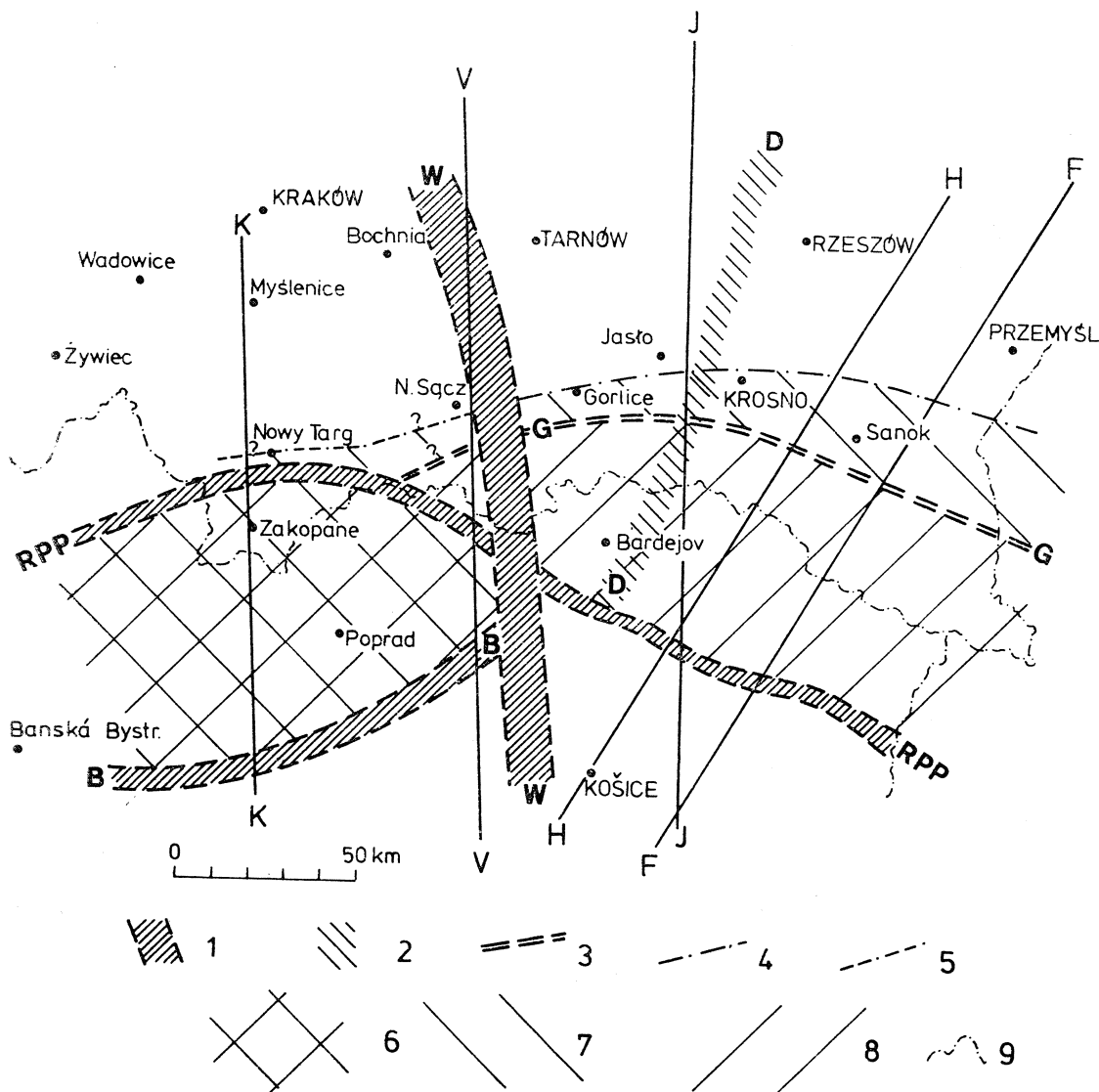
Fig. 4. Tectonic sketch-map of crustal structure in Polish Carpathians. 1 — fracture zones ( RPP — Peripienine fracture zone); 2 — probable tectonic zones; 3 — G—G line — northern boundary of the oceanic crustal fragment in the northern plate; 4 — northern boundary of the lowered fragment of Earth crust; 5 — inferred northern boundary of the lowered fragment of Earth crust; 6 — area of thickened crust in southern plate; 7 — lowered crustal fragment; 8 — area of oceanic crustal fragment in northern plate; 9 — state boundary. V—V — Vth International DSS Profile, F—F — Baligród—Radymno profile, H—H — Jaśliska—Błażowa profile. Profile symbols as in Fig. 1
