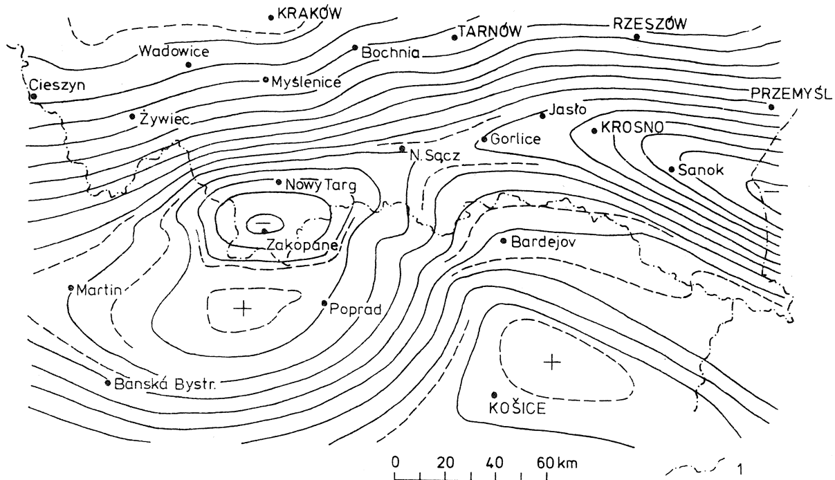
Fig. 9. Map of calculated gravity effect of three-dimensional model. Contour distance — 5 milligals. 1 — state boundary
