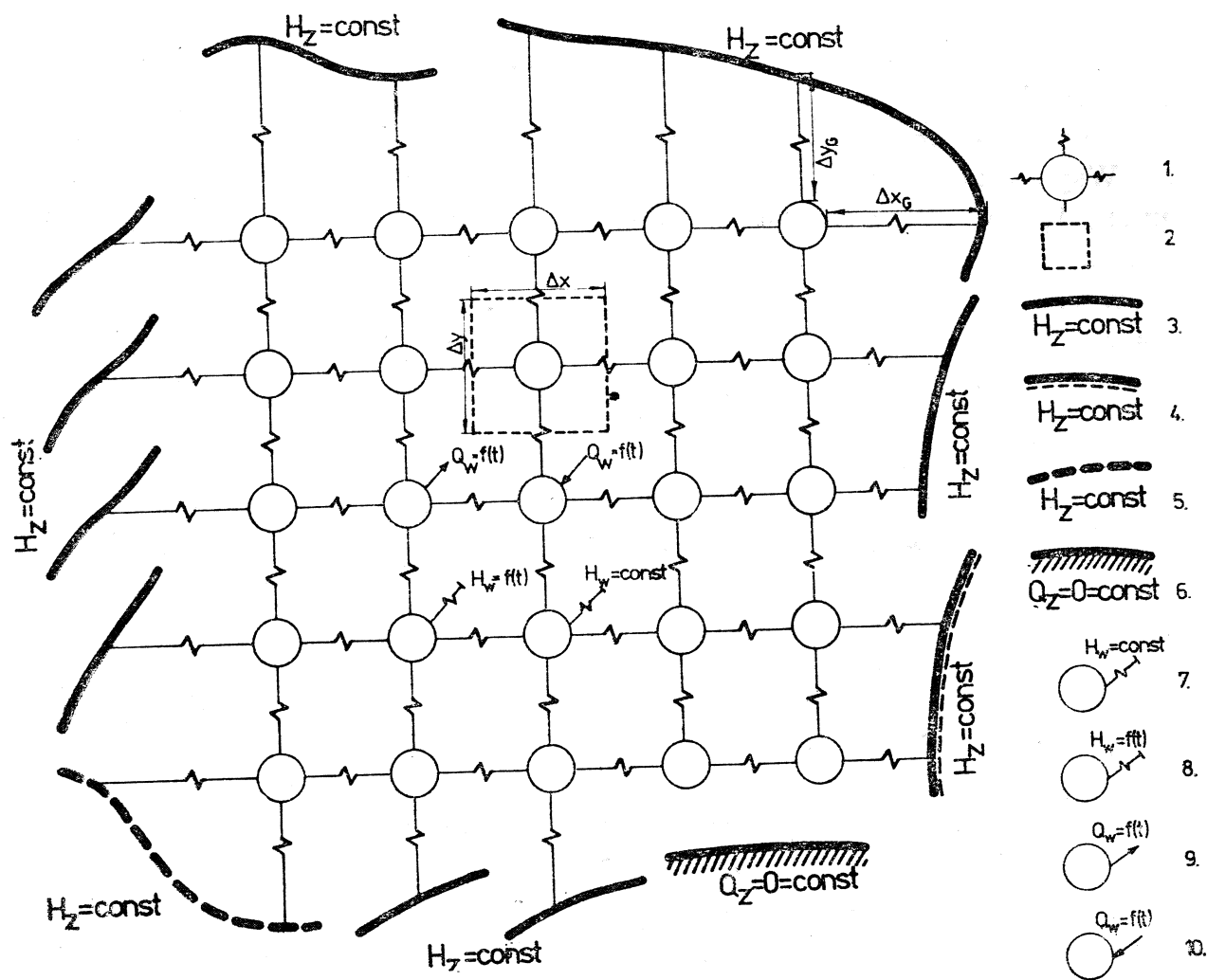
Fig. 3. Diagram of boundary conditions in the sectors of the investigated area. 1 — net junction of field analyser (knot) corresponding to the center of gravity of the calculation block; 2 — calculation block where \Delta x and \Delta y are the lengths of the block sides; 3 — external boundary condition of the 1st kind (contour of the constant hydraulic head); 4 — external boundary condition of the 1st kind, corresponding with the hydraulic head isoline contour of the hydraulic contact zone of Devonian and Triassic; 5 — external boundary condition of the 1st kind, hydraulic head varies along outcrops of carbonate Triassic under the Quaternary; 6 — external boundary condition of the 2nd kind, impermeable fault zone; 7 — internal boundary condition of the 1st kind, hydraulic contact with river B, with respect to the supposed karst solution channel or cavern passages system in the Triassic; 8 — internal boundary condition of the 1st kind, erosional hydraulic contact of the Triassic with the Quaternary; 9 — internal boundary condition of the 2nd kind, ground-water extraction from Triassic aquifer by ore mines and municipal water supplies; 10 — internal boundary condition of the 2nd kind, indirect recharge of the Triassic aquifer from Jurassic or Devonian
