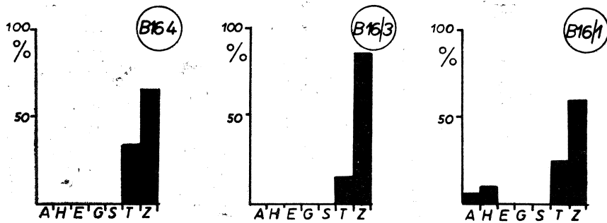
Fig. 4. Percentages of heavy minerals related to their order of persistence (stability to weathering). Letter symbols as in Fig. 3
