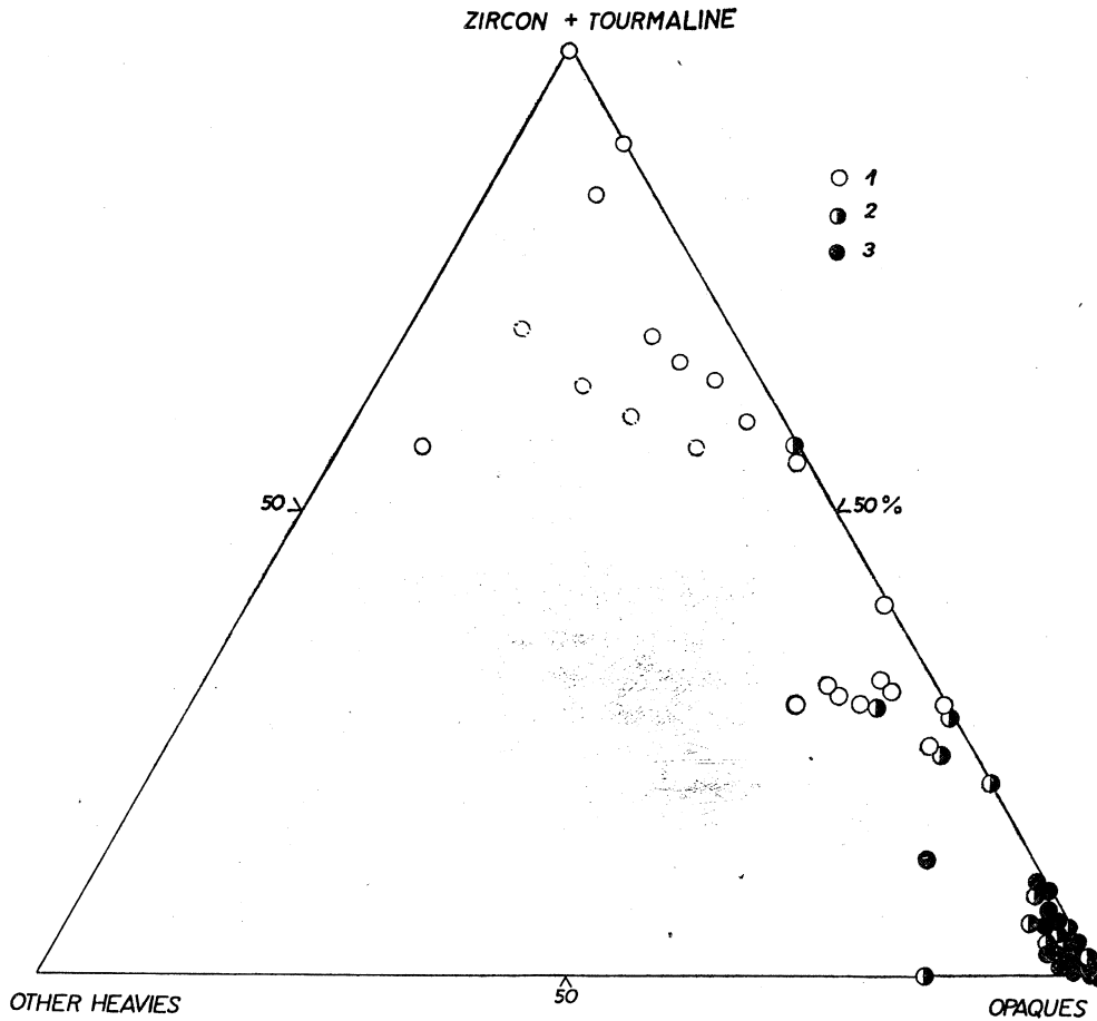
Fig. 5. Modal composition of heavy fraction, Permian sandstones. 1 — white „structureless” ss., 2 — white cross-stratified ss., 3 — red cross-stratified ss.
