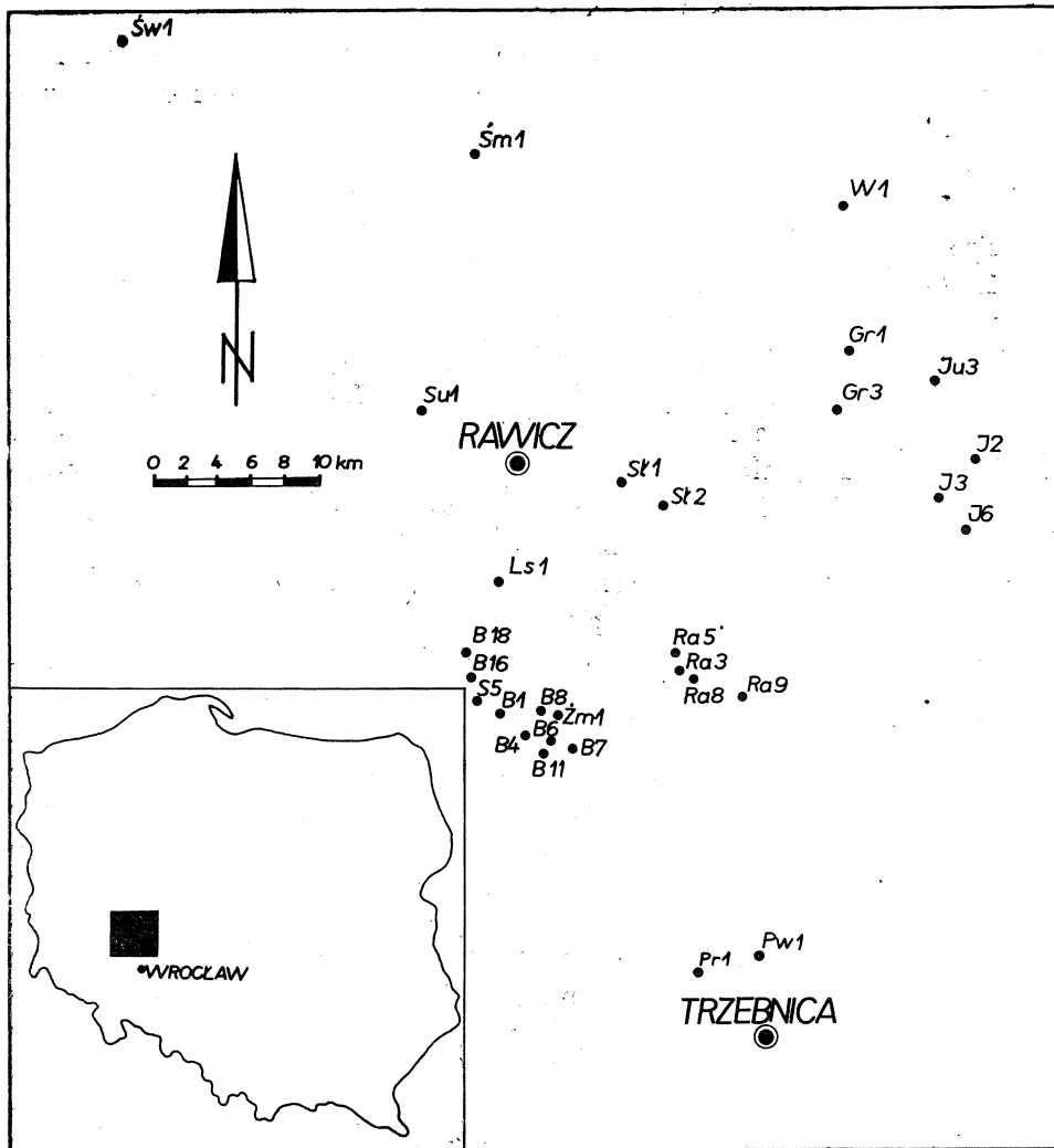
Fig. 2. Index map showing location of bore-holes
