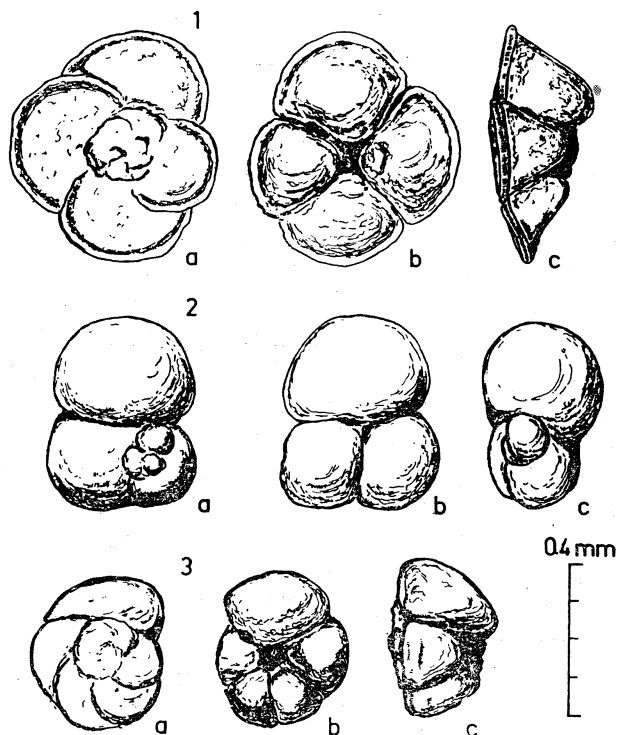
Fig. 4. Planktonic foraminifers from the Middle Paleocene at Szaflary. 1a—c — Globorotalia angulata (White); 2a—c — Globigerina triloculinoides Plummer; 3a—c — Globorotalia aequa Cushman et Renz
