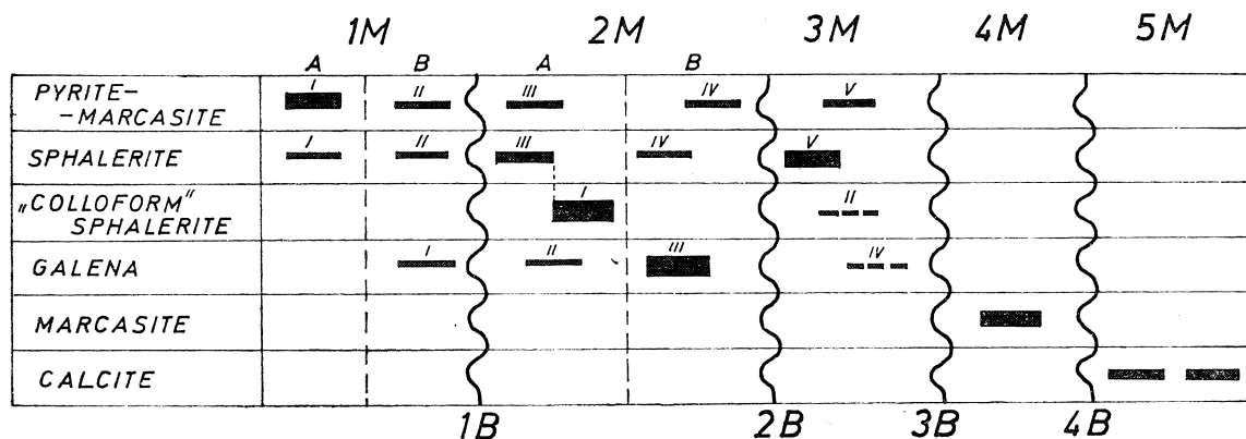
Fig. 2. Paragenetic diagram for Olkusz ores
