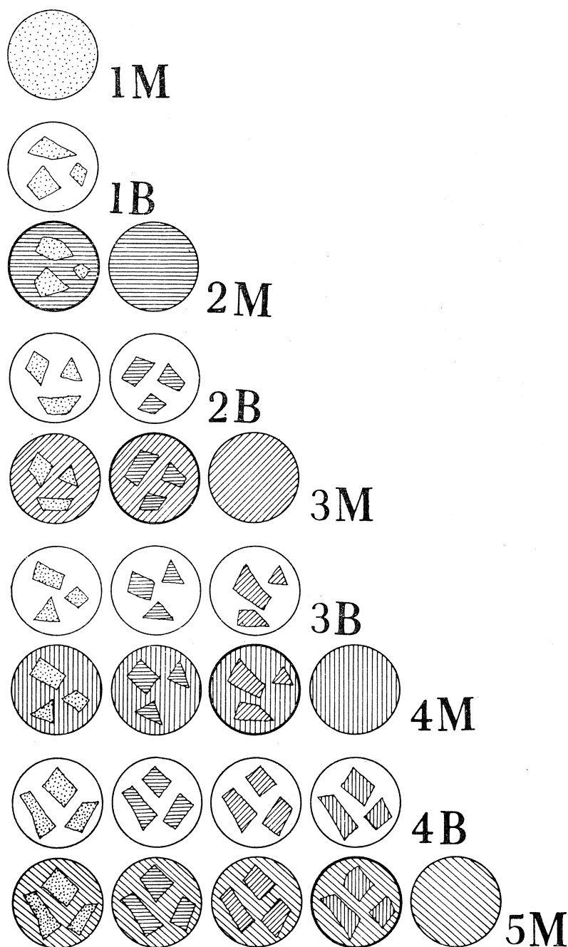
Fig. 1. Schematic diagram illustrating development of mineralized breccias. 1M, 2M, 3M, 4M and 5M — stages of mineralization; 1B, 2B, 3B and 4B — stages of brecciation. Products of earlier mineralizations are enveloped by younger minerals. Each stage of mineralization is marked by different design. Circles delineated by thick lines correspond to structures shown in Pl. I. Fig. 1, 2 and Pl. II. Fig. 1, 2
