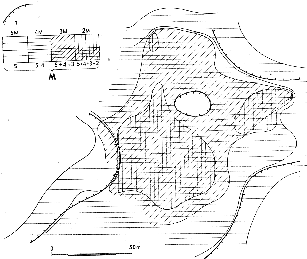
Fig. 4. Horizontal section of breccia structure showing distribution of products of various stages. 1 — breccia boundary. Design in rectangular inset (upper left) indicated by 2M, 3M, 4M, 5M correspond to different mineralization stages; numbers 5+4, 5+4+3 and 5+4+3+2 correspond to superposition of different stages
