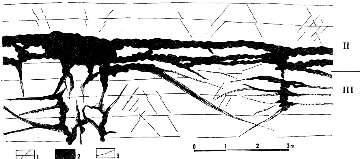
Fig. 8. Replacement structures in zone II and cavity-filling structures in zone III (compare fig. 6 B). 1 — ore-bearing dolomite; 2 — galena II and III; 3 — colloform sphalerite I
