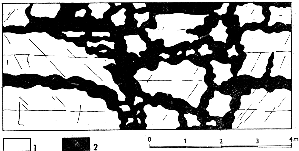
Fig. 7. Replacement structures observed in II zone of generalized profile shown in fig. 6 B. 1 — ore-bearing dolomite; 2 — galena III
