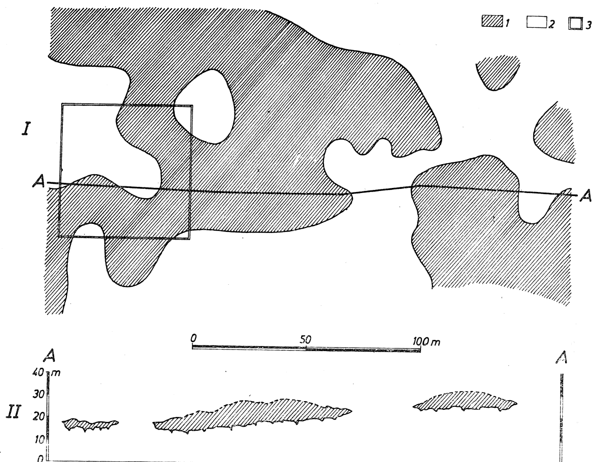
Fig. 5. Horizontal plan view of ore nests (I). Vertical section along line A—A (II). 1 — breccia; 2 — undisturbed ore-bearing dolomite; 3 — area illustrated by cross-section — fig. 6
