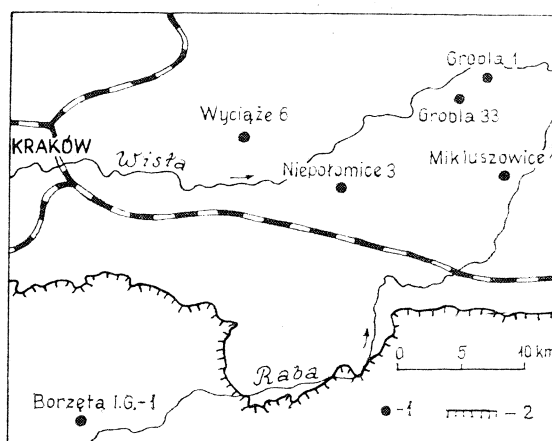
Fig. 1. Index map showing location of bore-holes discussed in the text, 1 — bore-holes; 2 — margin of the Carpathian overthrust
