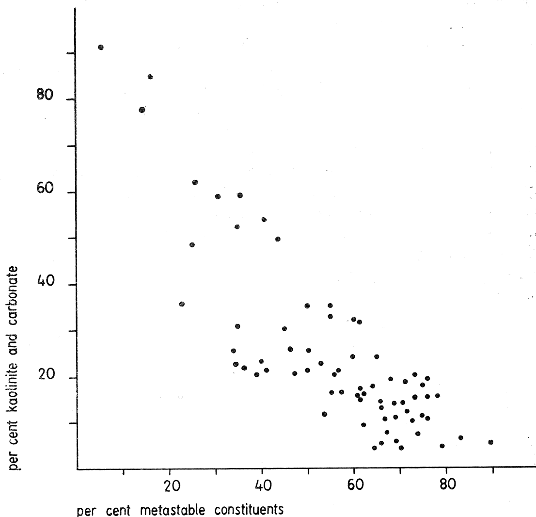
Fig. 1. Showing content of kaolinite and carbonate versus metastable detrital components in Lower Carboniferous deposits from the western Intrasudetic Basin. Data from concretionary bodies cluster in the upper half of the figure, whereas that from carbonate-cemented sandstones are grouped in the lower half. Samples involved were originally carbonate-free and their kaolinite content was low. Based on thin section data
