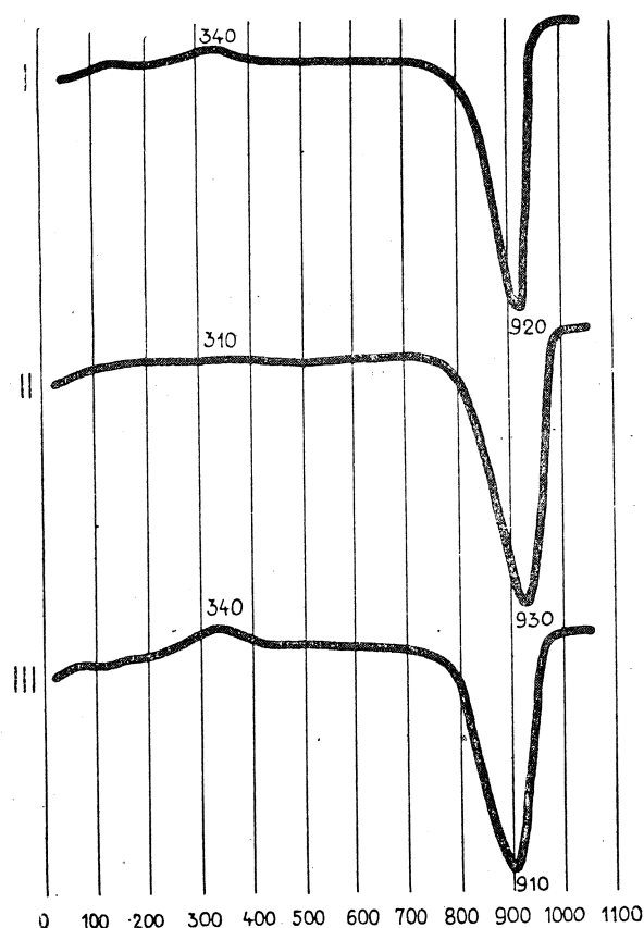
Fig. 2. DTA diagrams of oncolites. Diagrams I and II — oncolites of North Vietnam, I — porous layer, II — compact layer, III — diagram of an oncolite of the Tatra Mts.
