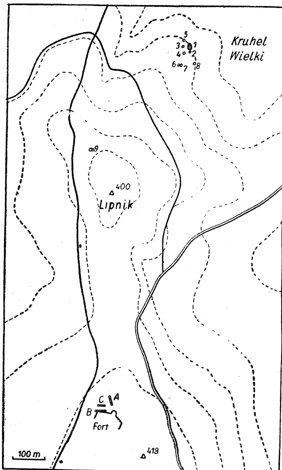
Fig. 1. Map of the vicinity of Przemyśl Fort — old fortifications on the hill 413 with outcrops described in the text; S — Jurassic klippes
