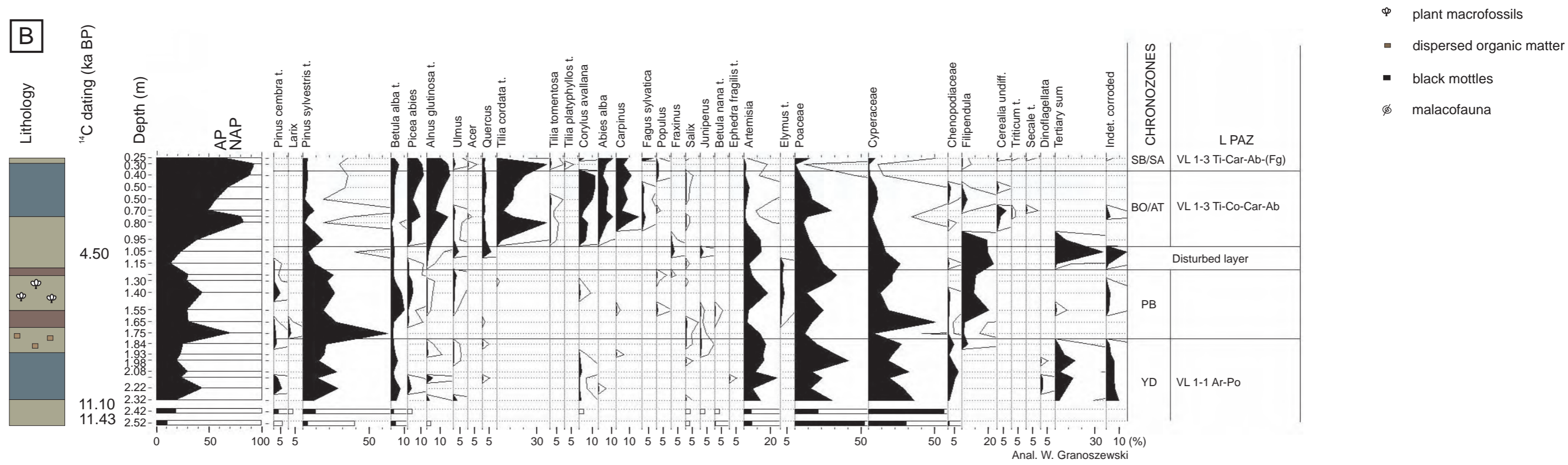
Fig. 3. Pollen diagrams from (A) borehole No. 4' and (B) outcrop VL-1
