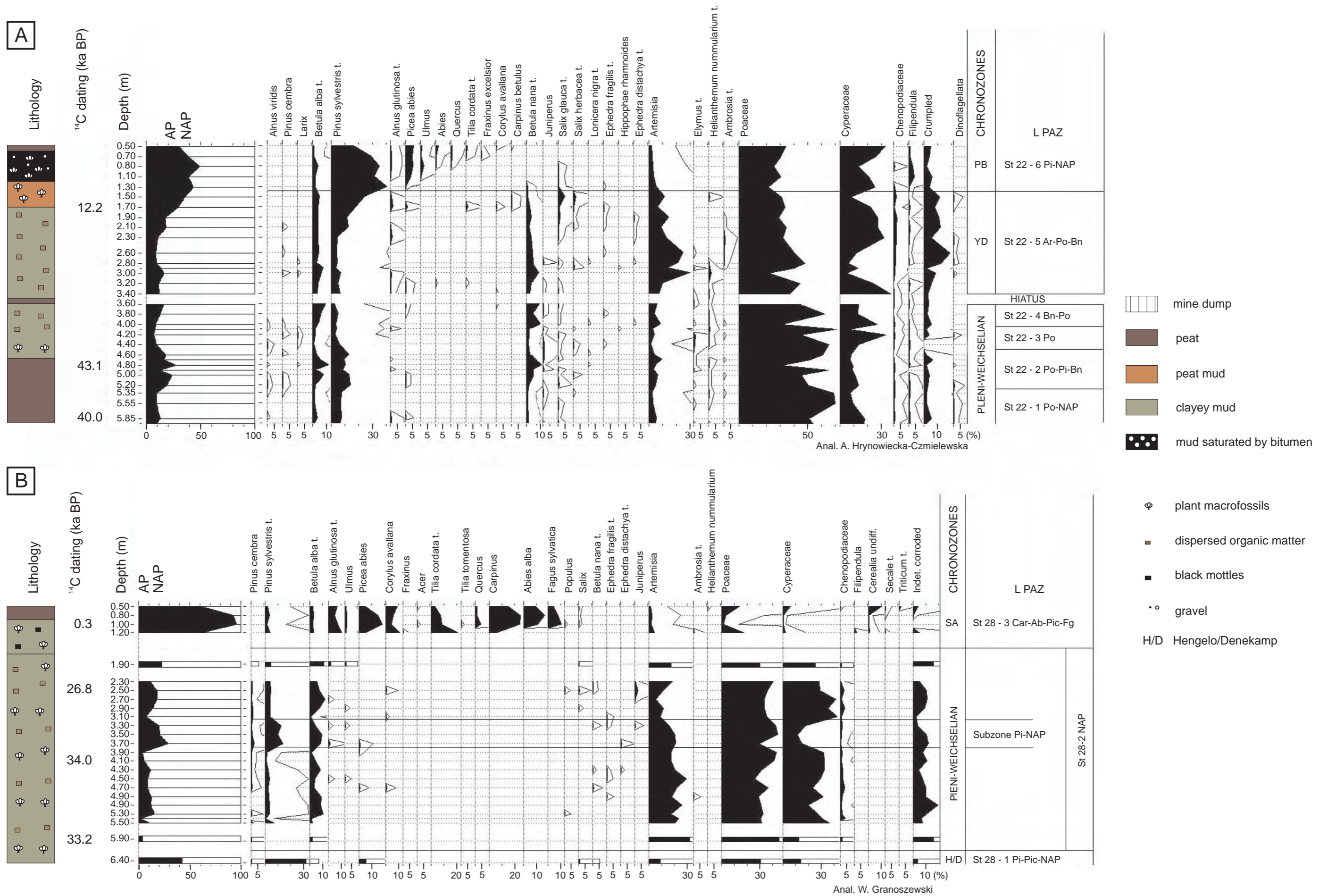
Fig. 2. Pollen diagrams from boreholes (A) No. 22 and (B) No. 28
