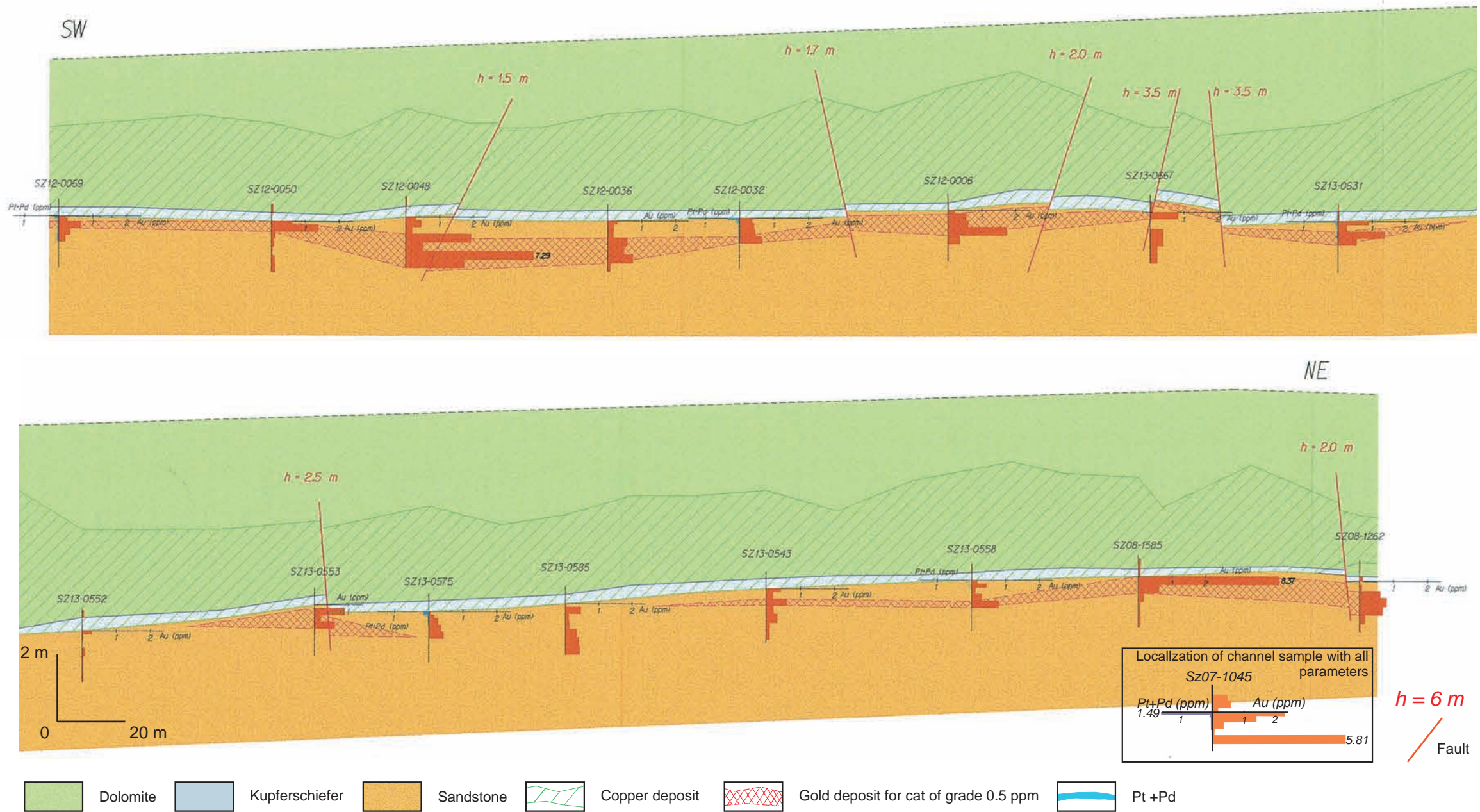
Fig. 84. Cross section P5u along mining work I-5, Polkowice Mine, East Field
